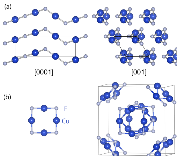
Fig. 1 (a) The predicted bulk crystal structure of CuF (space group 154, a = 3.29 Å, c = 9.16 Å); (b) the tetramer building block of CuF nanoclusters, and the corresponding cubic tetramer network.
