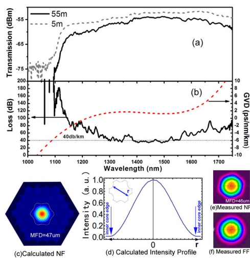
Fig. 2. (Color online) (a) Fiber optical transmission spectra. (b) The fiber optical attenuation spectrum (solid black curve) and calculated GVD (dashed red curve). The dotted horizontal curve shows the baseline of the attenuation figure. (c) Calculated near-field (NF) pattern with an MFD of 47 \mu\text{m} . (d) Calculated intensity profile showing along the axis shown in the top left insert. (e) Measured NF pattern showing. (f) Measured far-field (FF) pattern.
