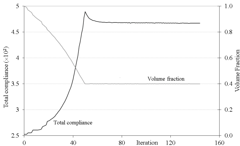
Figure 13. Beam optimization for multiple load cases, convergence history.
