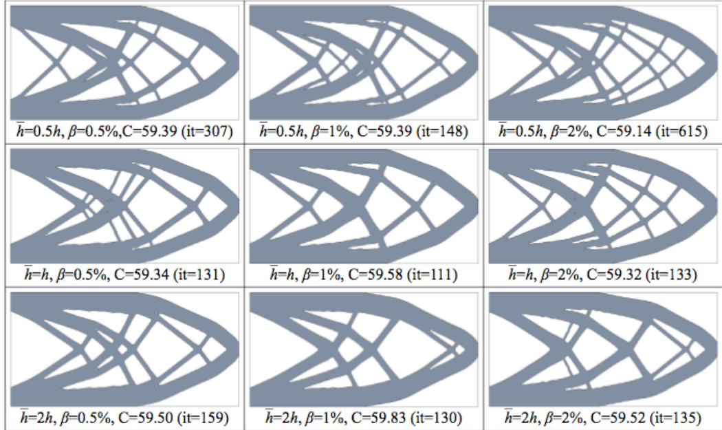
Figure 5. Cantilever beam solutions for band width, \omega = 4h . Compliance values, ( C, \times 10^2 ) are for final solution at the iteration (it) shown.
