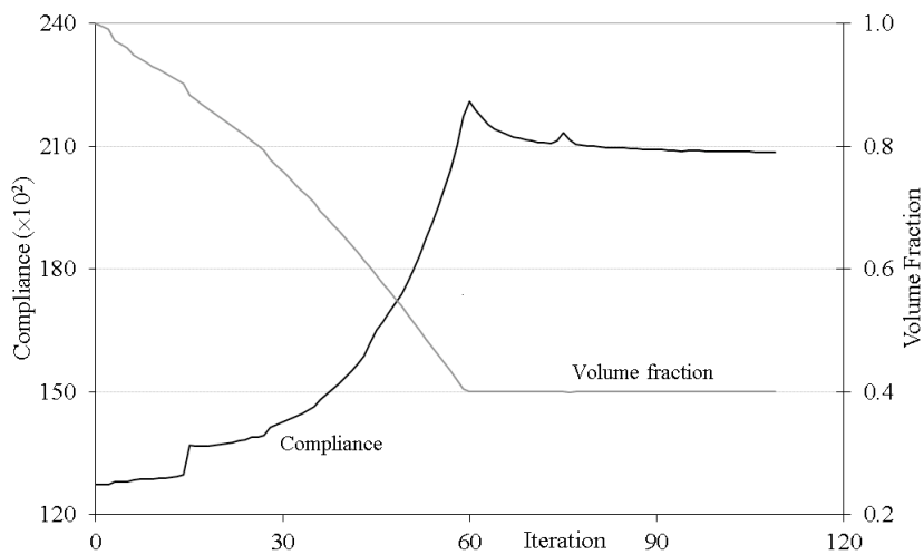
Figure 10: MBB beam, convergence history.
