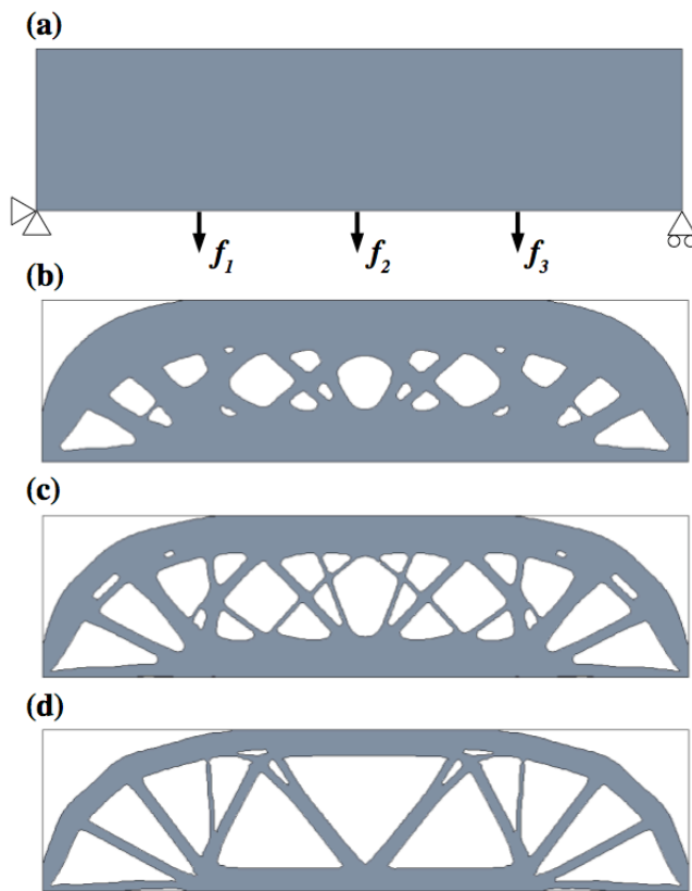
Figure 12. Beam optimization for multiple load cases: (a) initial design and boundary conditions; (b) design after 25 iterations; (c) 40 iterations; (d) converged solution after 144 iterations.
