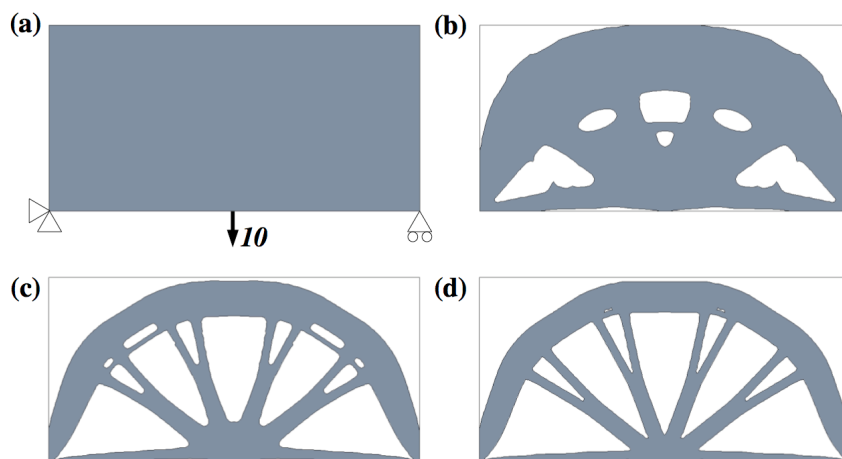
Figure 7. Michell structure: (a) initial design and boundary conditions; (b) design after 35 iterations; (c) 70 iterations; (d) converged solution after 107 iterations.
