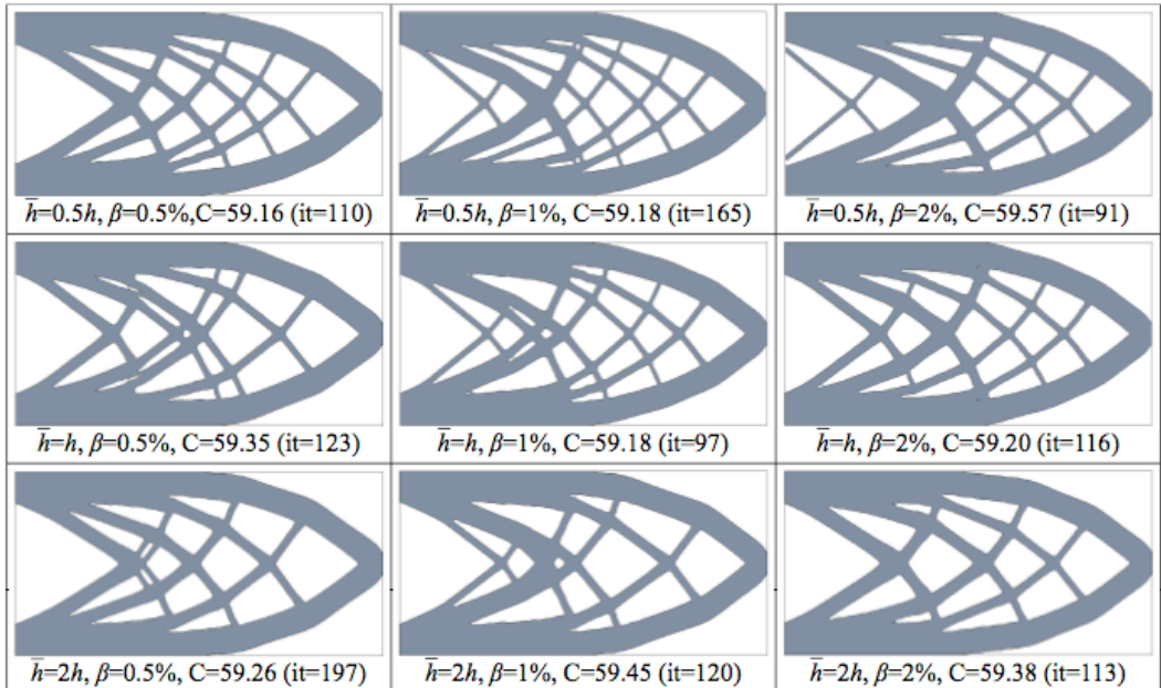
Figure 6. Cantilever beam solutions for band width, \omega = 6h . Compliance values, ( C, \times 10^2 ) are for final solution at the iteration (it) shown.
