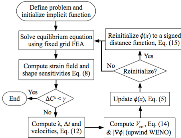
Figure 1. Level set optimization algorithm flowchart.
