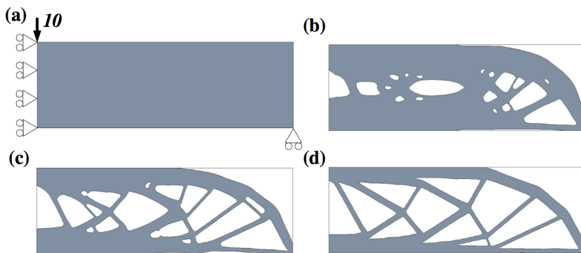
Figure 9. MBB beam: (a) initial design and boundary conditions; (b) design after 30 iterations; (c) 50 iterations; (d) converged solution after 109 iterations.
