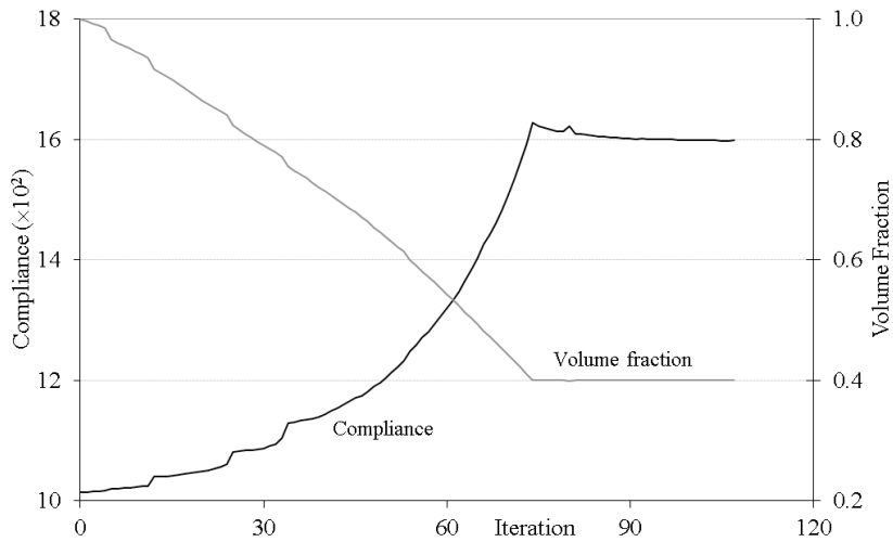
Figure 8. Michell structure, convergence history.
