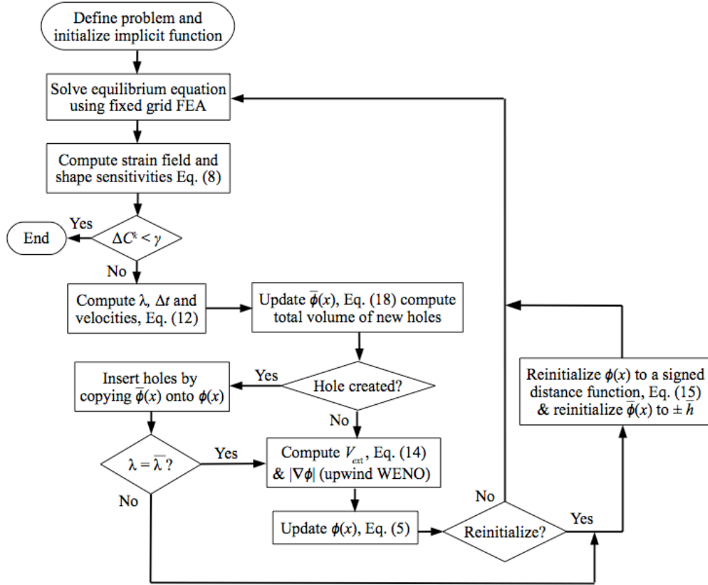
Figure 3. Level set optimization algorithm flowchart with hole insertion.
