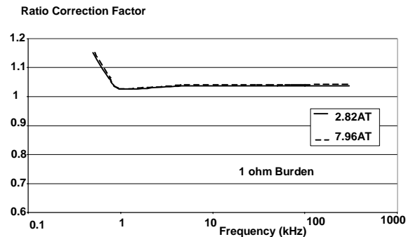
Figure 7. Ratio Correction Factor Vs Frequency Current Transformer Class X 800/1 191 V knee point.
