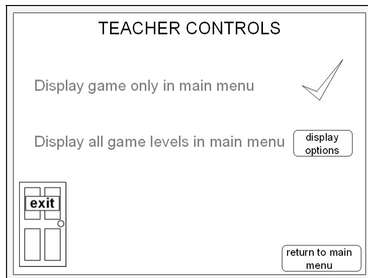
Figure 8 – teacher controls
