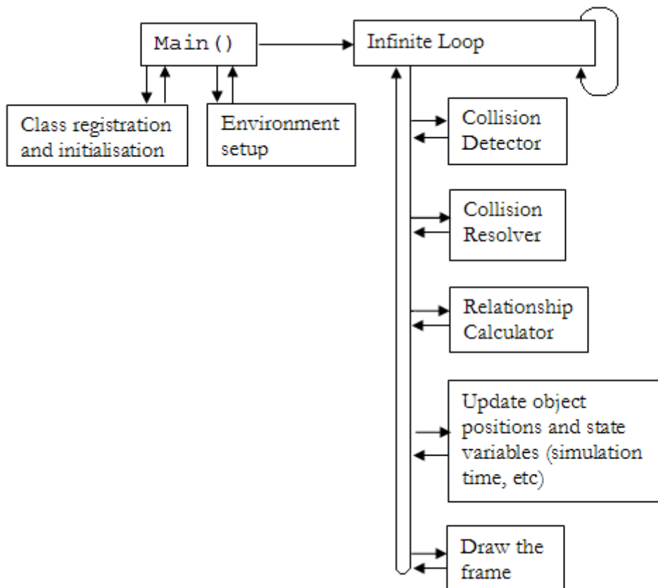
Figure 1: Program Flow
