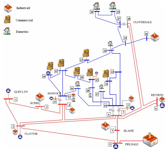
Fig 5. The IEEE 30 Bus Test System with different types of demand
