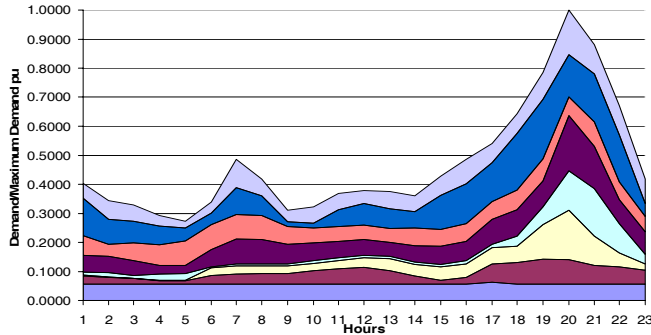
Fig 3. Single Tariff Domestic Demand
