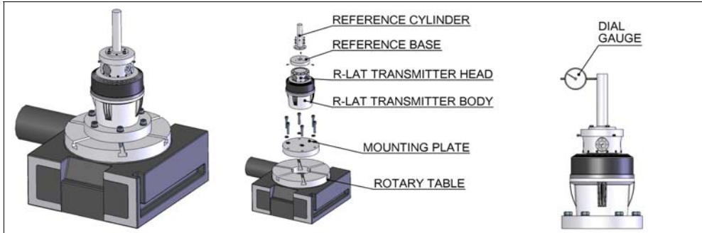
Figure 3: Experimental Setup
