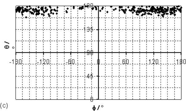
Fig. 6 QM/MM MD simulation for Model 1 in water: (a) plot of composite angle \phi vs. time and (b) conformational space sampled during the QM MD trajectory for xylose ring conformation starting from {}^{2.5}B conformation; (c) conformational space sampled starting from {}^4C_1 conformation.
