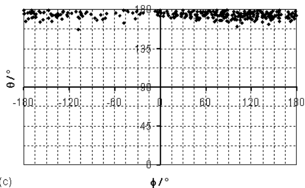
Fig. 7 QM/MM MD simulation for Model 2: (a) plot of composite angle \phi vs. time and (b) conformational space sampled during the QM MD trajectory for xylose ring conformation starting from {}^{2.5}B conformation; (c) conformational space sampled starting from {}^4C_1 conformation.
