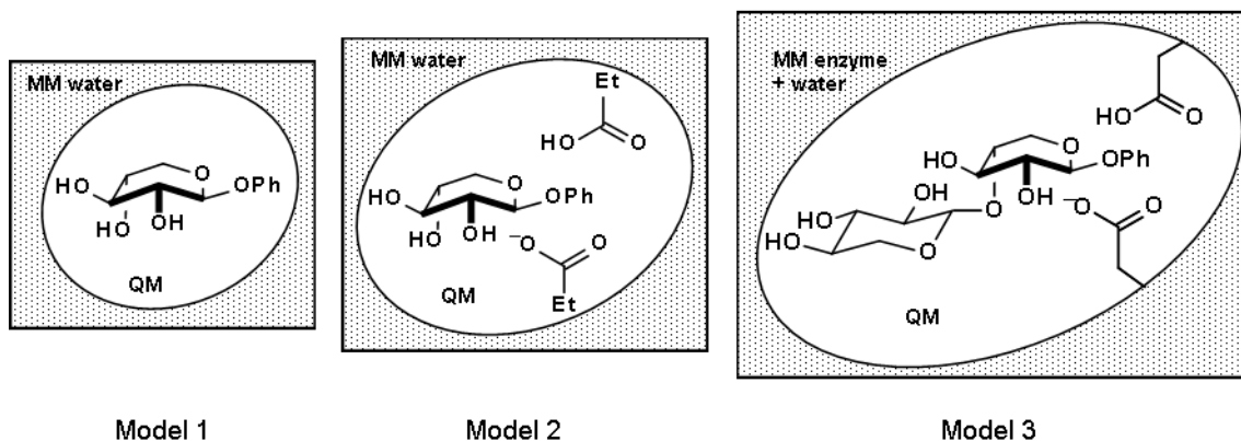
Fig. 3 Schematic representations for models 1, 2 and 3.
