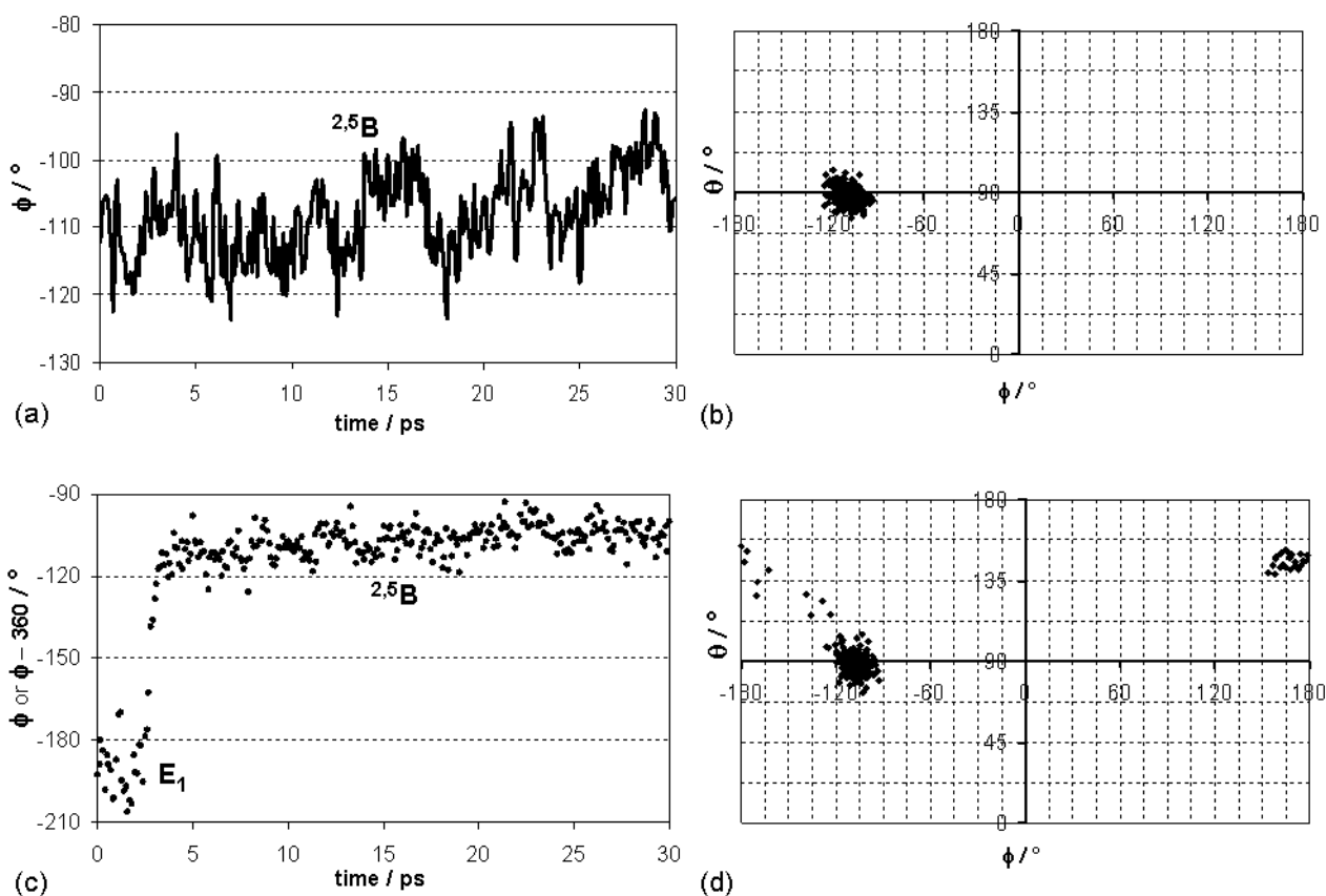
Fig. 9 QM/MM MD simulation for Model 3: (a) plot of composite angle \phi vs. time and (b) conformational space sampled during the QM MD trajectory for xylose ring conformation starting from ^{2,5}B conformation; (c) plot of \phi vs. time and (d) conformational space sampled starting from ^4C_1 conformation.
