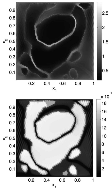
FIG. 9. Elastic energy density (top panel) and order parameter \rho_0 (bottom panel) of the fully relaxed state of a simulation with initial and boundary conditions on a rank-1 connection in between the tetragonal and the monoclinic minima of the energy. A complex arrangement of phases has formed, with boundaries of higher energy in between.
