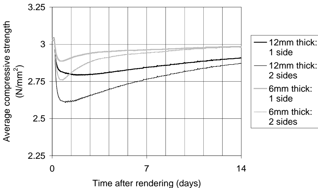
Figure 7: Effect of rendering on average unit compressive strength
