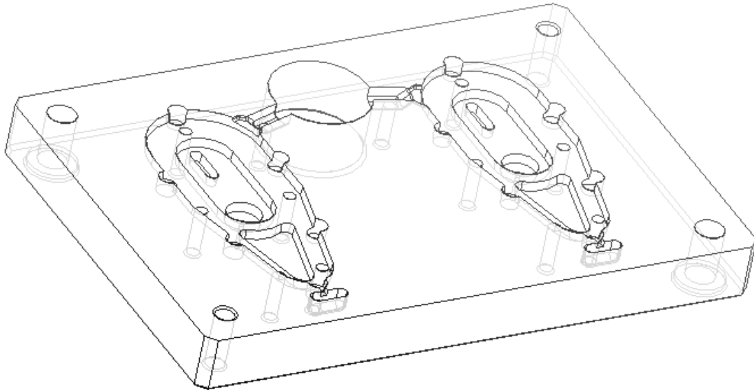
Figure 1 Twin cavity casting die for mounting plate
