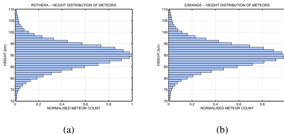
Fig. 4. Normalised variation of meteor counts with height for the (a) Rothera meteor radar between 2005 and 2009 and (b) Esrangle meteor radar between 1999 and 2009.
