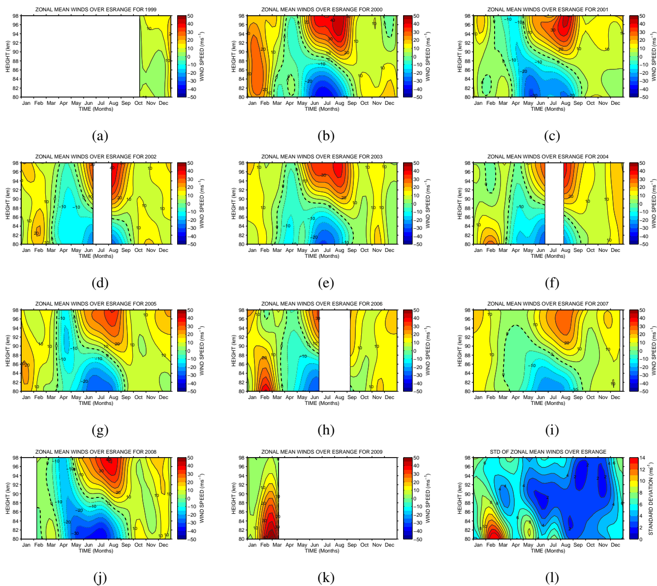
Fig. 7. (a–k) Monthly-mean zonal winds measured by the ESRANGE meteor radar for individual years between 1999 and 2009. (l) The standard deviation of all years of monthly-mean zonal winds.
