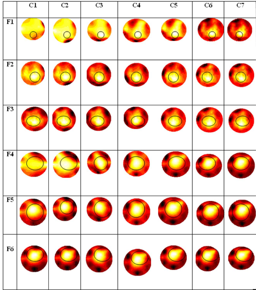
Fig. 5. Temporal image. Each row includes seven images for excitation coils 1–7. The six rows represent the six flow regimes shown in Fig. 4. In these images, the bright area represents the molten steel flow, whereas the dark area represents the surrounding air.
