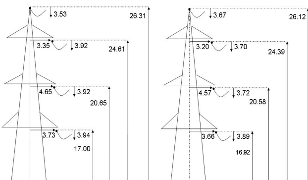
Fig. 12a. Double circuit towers, from left to right: Beaulay to Boat of Garten OHL and Beaulay to Keith via Nairn OHL, geometric configuration, showing horizontal and vertical placement, conductor positioning and conductor sag at mid span.
