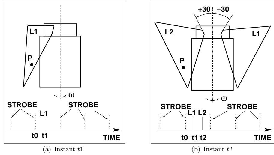
Figure 2. Schema of a transmitter at the instants t_1 and t_2 when the first and the second fanned beam respectively intersects the position of a sensor (P). -30 and +30 are two arbitrary values of the slant angles.
