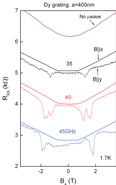
FIG. 9: Comparison of the photoresistance obtained in a transverse magnetic field ( B_a \parallel y ) and a longitudinal magnetic field ( B_a \parallel x ) for sample B . When B_a \parallel x , the dipolar magnetic field is zero. Resonant absorption is recovered by aligning B_a \parallel y .
