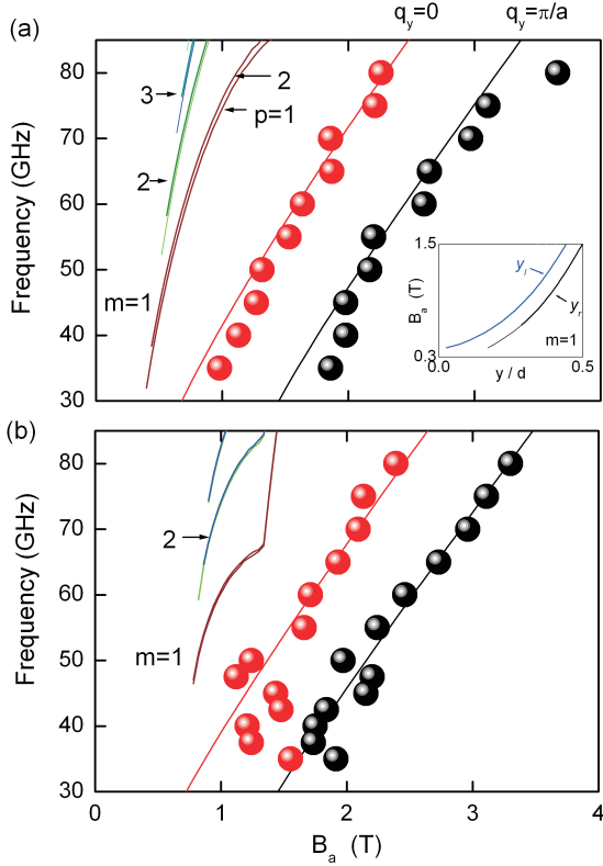
FIG. 12: Theoretical frequency dependence of the DESW modes ( m=1,2,3\dots p=1,2 ) in samples (a) C and (b) B . The theoretical frequency dependence of the onset and cutoff magnetic fields of the DMW band is plotted as the red and black curves. Inset: left and right turning points of the m=1 DESW mode. The spin wave drifts towards the edge of the stripe as the magnetic field increases.
