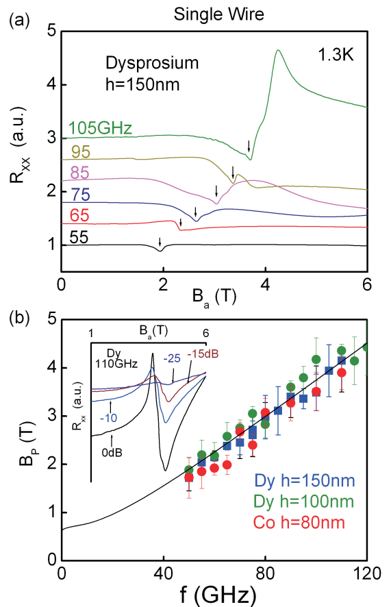
FIG. 2: (a) Ferromagnetic resonance of sample A detected through a change in the resistance of the 2DEG ( B_a \parallel y ). Curves are vertically offset for clarity. (b) Frequency dependence of the resonant field (symbols) fitted with Eq.1 (full line). Inset: microwave power dependence.
