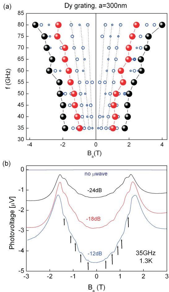
FIG. 7: (a) Frequency dependence of the microwave resonances in the photovoltage of sample C . The fan diagram shows the FMR onset (red dots), the FMR cutoff (black dots) and the frequency dependence of the small photovoltage dips at low field (blue circles). (b) Detail of the 35GHz curves showing the resonances with DESW modes and their dependence of microwave power.
