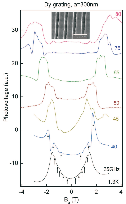
FIG. 6: Photovoltage spectroscopy of magnetic excitations in sample C ( B_a \parallel y ). The broad FMR peak corresponds to the excitation of DMWs across the grating. The series of dips highlighted by the arrows indicates resonances with quantized DESW modes in individual stripes. Curves are vertically offset for clarity. Inset: dysprosium grating of sample C (detail).
