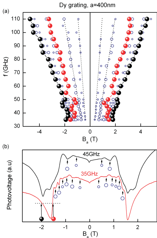
FIG. 5: (a) Frequency dependence of the microwave resonances in the photovoltage of sample B . The fan diagram shows the FMR onset (red dots), the FMR cutoff (black dots) and the dependence of the small photovoltage dips at low field (blue circles). (b) Details of the fine resonant structure at 35GHz and 45GHz. The diameter of the blue circles is proportional to the amplitude of the dips. The onset (red dot) and the end (black dot) of the FMR range are defined at the mid-height of the main resonance.
