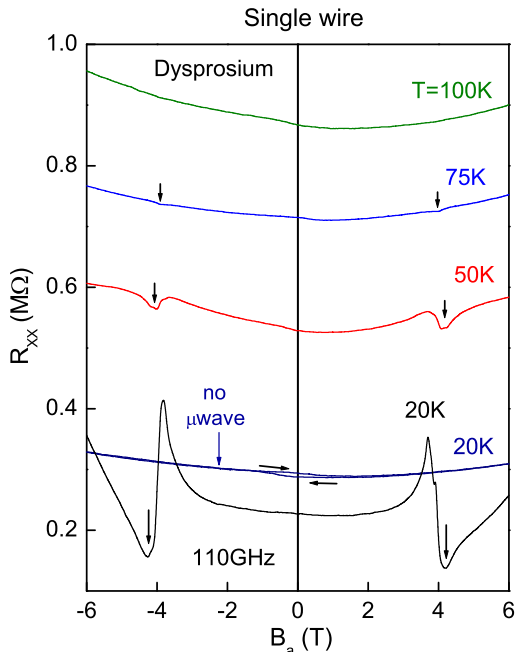
FIG. 3: Temperature dependence of the photoresistance of sample A. The FMR vanishes above the Curie temperature of dysprosium (85K). The magnetic hysteresis of dysprosium is visible in the curves measured without microwaves. Other curves are measured by sweeping the magnetic field up.
