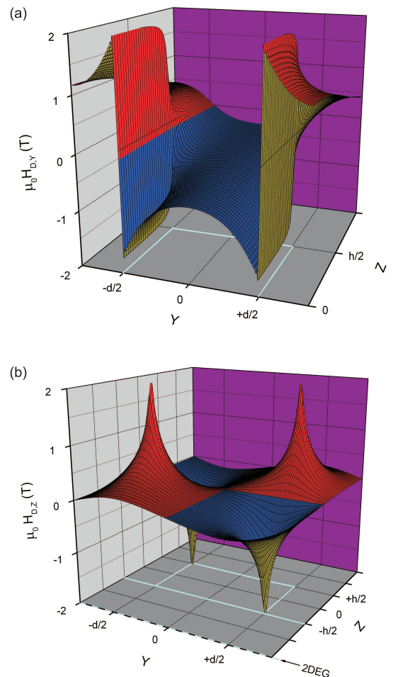
FIG. 10: Spatial variation of the (a) in-plane and (b) perpendicular dipolar magnetic field in one stripe of superlattice C . The superlattice is assumed to be magnetized to saturation along y . The edges of the stripe are indicated by the full lines in the (y,z) plane. The magnetic field that couples the grating to the 2DEG is the sine wave at the fore of panel(b).
