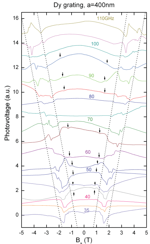
FIG. 4: Photovoltage spectroscopy of magnetic excitations in sample B ( B_a \parallel y ). The dotted lines are a guide to the eye for the magnetic field dependence of the onset and the cutoff of the FMR range. At lower magnetic field, the arrows indicate a series of smaller dips induced by microwaves. Curves are vertically offset for clarity. Parameters: a = 400 nm, d = 200 nm, h = 160 nm, T = 1.3 K.
