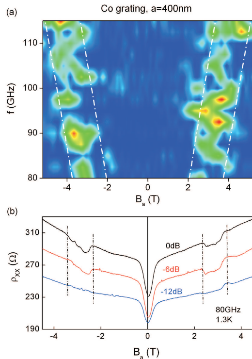
FIG. 8: (a) Photoresistance of sample D mapped as a function of microwave frequency and magnetic field ( B_a \parallel y ). The bandwidth of the resonance with DMWs is delimited by the dash-dotted lines. (b) Microwave power dependence.
