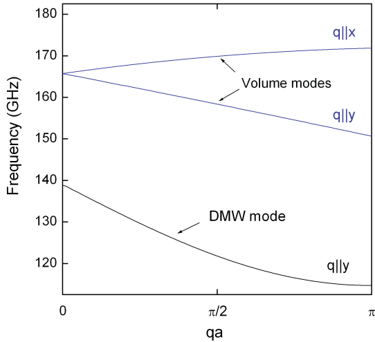
FIG. 13: Frequency dispersion curve of dipolar magnetization waves in superlattice C at B_a = 5T . The volume spin wave modes of a 80nm thick dysprosium film are also shown for the two directions of propagation, parallel ( q||y ) and perpendicular ( q||x ) to the magnetization.
