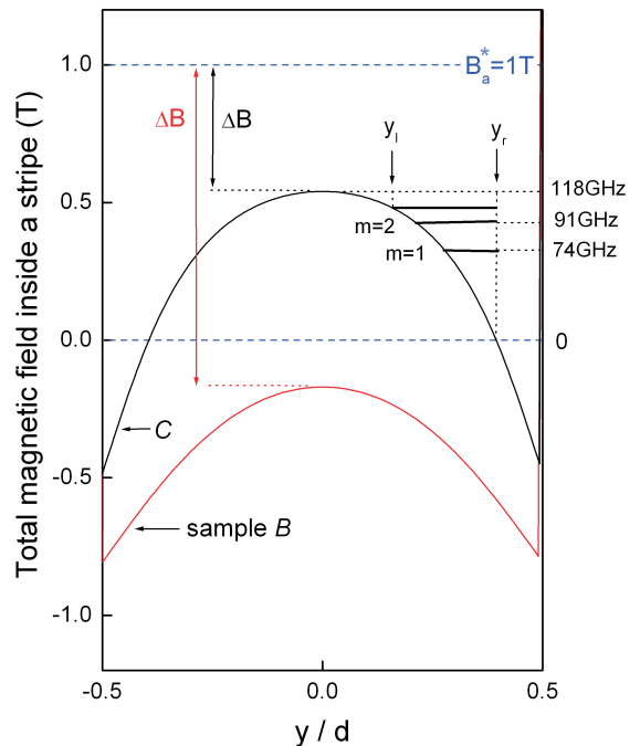
FIG. 11: Internal magnetic field across one stripe at height z=0 . The magnetic bias is B_a + \bar{B}_h = 1\text{T} . \Delta B is the bias threshold where the internal magnetic field becomes positive at the centre of the stripes and starts squeezing spin waves against the edges. The quantized DESW modes m=1,2 and 3 ( p=1 ) are shown together with their frequencies. y_l and y_r are the left and right turning points of the m=3 DESW mode.
