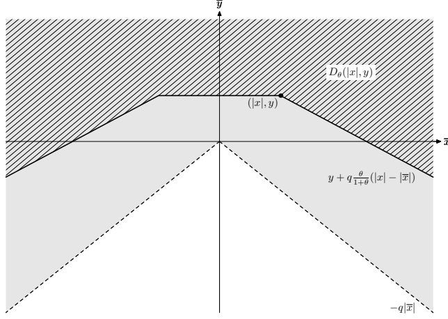
Figure 3: The point process \Pi is defined on the set \widehat{H} indicated in grey. If we fix Z_t/r_t = x, \Phi_t(Z_t)/a_t = y , the condition that Z_t = Z_{t+\theta t} corresponds to the requirement that the point process \Pi has no points in the shaded region D_\theta(|x|, y) .
