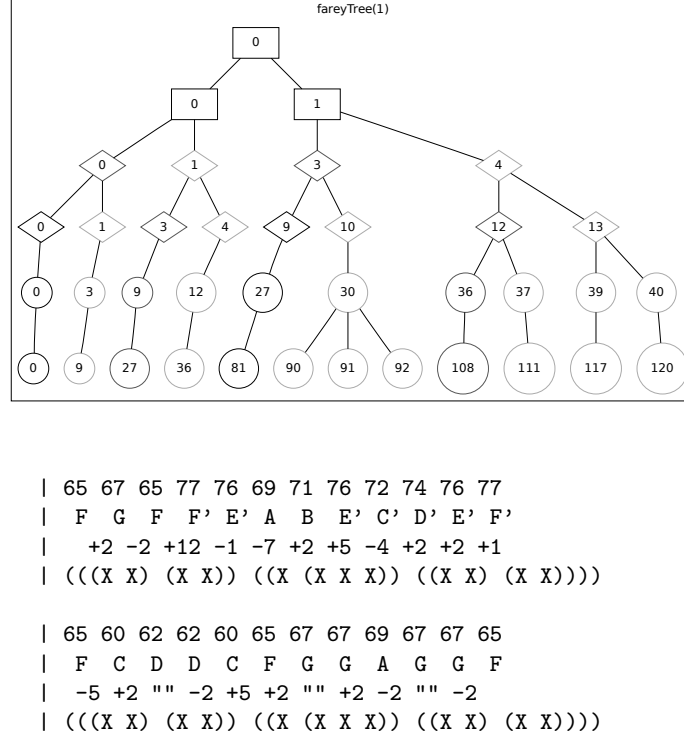
Fig. 10. The partitioning tree and human readable format for the Lydian duet composition.
