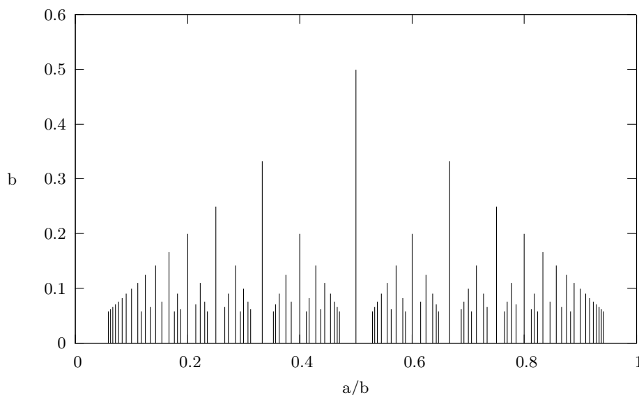
Fig. 8. Correlation of a/b \in F_{17} and 1/b in the interval (0, 1)
