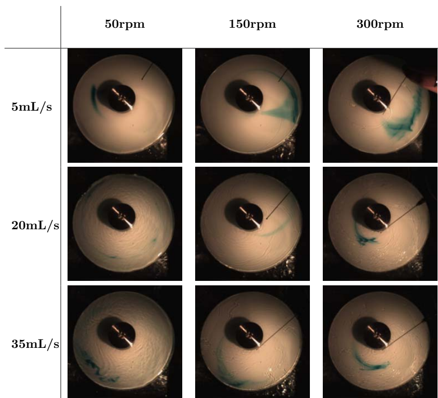
Figure 4: High speed camera images of the spinning disc with dye injected at the inlet.
