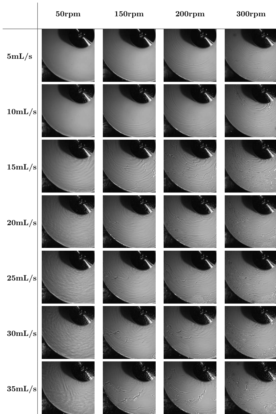
Figure 2: High speed camera images of the spinning disc fed water at various flow rates and disc rotational speeds.
