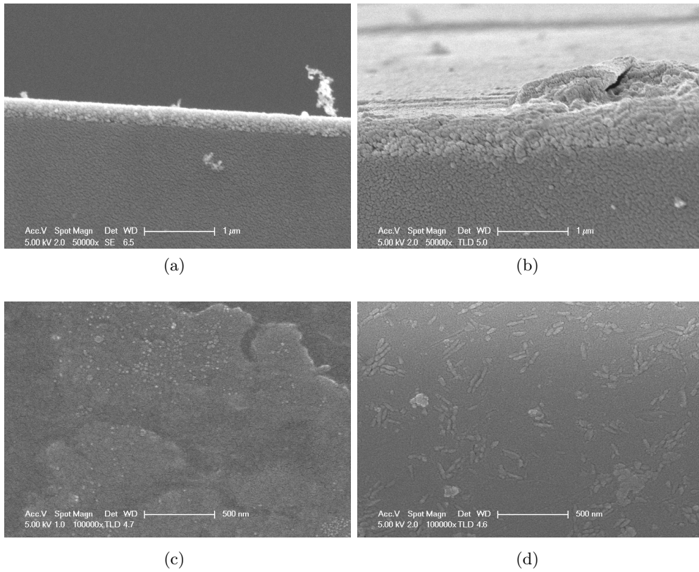
Figure 6: SEM images of titanium dioxide sol-gel coating: (a) cross-sectional view before reaction (b) cross-sectional view after reaction (c) front on view before reaction (d) front on view after reaction
