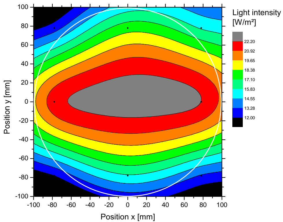
Figure 11: UV light intensity distribution on the glass disc in the spinning disc reactor, with white circle indicating the outside disc surface.
