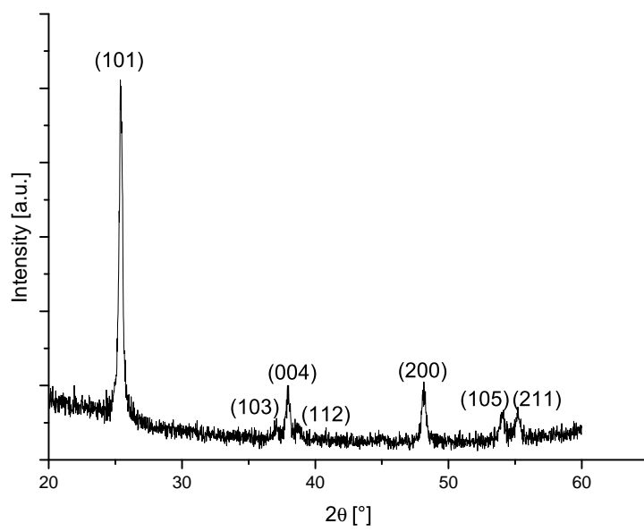
Figure 5: XRD spectrum of the TiO 2 coating.
