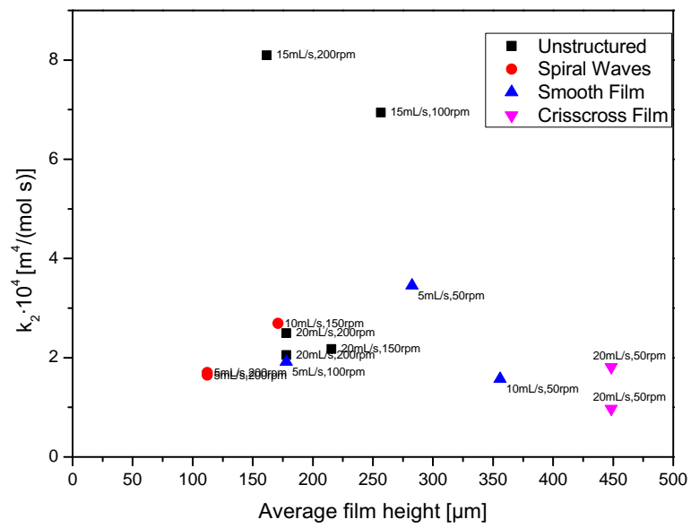
Figure 10: Effect of film height on the pseudo-second order surface area based reaction rate constants as classified by flow regime.
