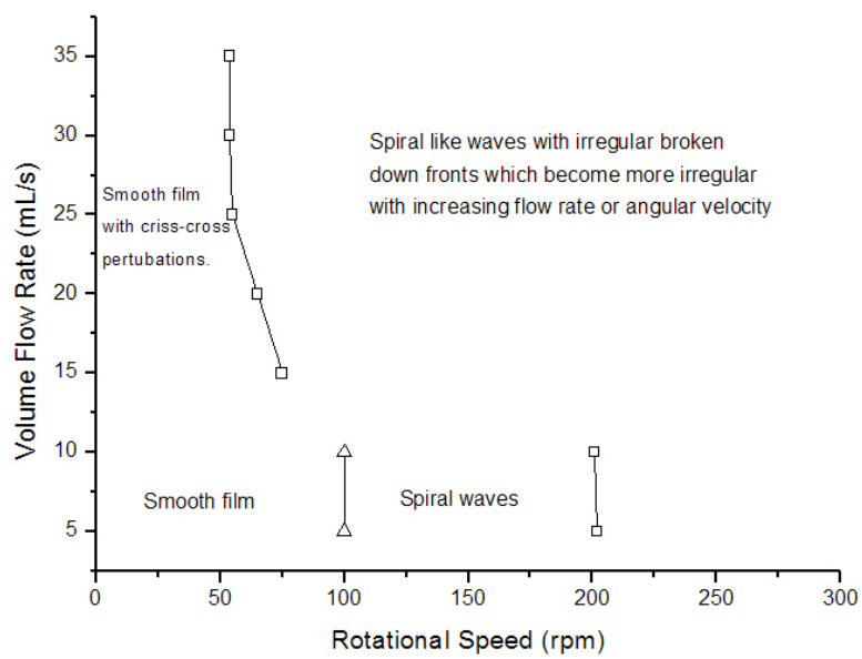
Figure 3: Flow regimes on the spinning disc reactor at different flow rates and rotational speeds.
