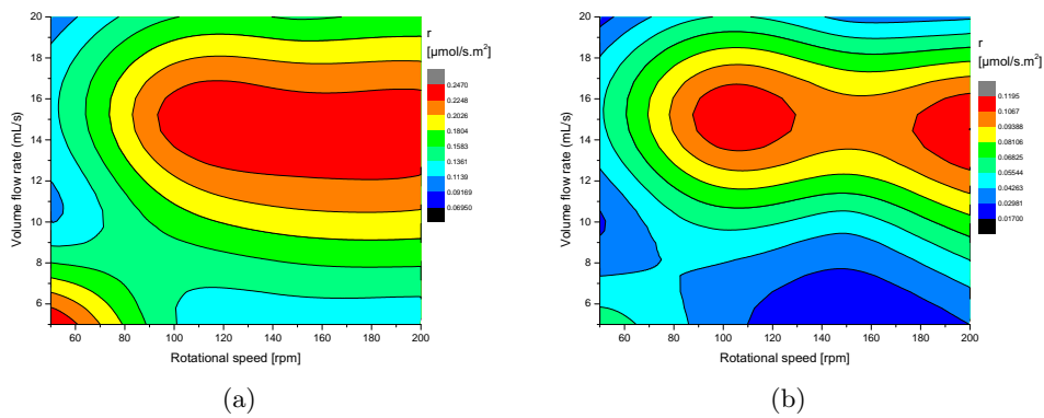
Figure 9: Calculated reaction rates at methylene blue concentrations of (a) 26 \mu\text{mol/L} and (b) 13 \mu\text{mol/L} .
