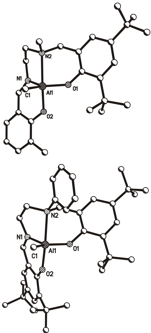
Fig. 1 Top: Molecular structure of Al(3)Me. Selected bond lengths ( \text{\AA} ) and angles ( ^{\circ} ) are Al(1)-O(1) 1.757(2), Al(1)-O(2) 1.827(2), Al(1)-C(1) 1.960(3), Al(1)-N(1) 1.979(3), Al(1)-N(2) 2.266(3), O(2)-Al(1)-O(1) 90.48(11) , O(2)-Al(1)-C(1) 99.65(14) , O(1)-Al(1)-C(1) 124.68(14) , O(2)-Al(1)-N(1) 89.51(12) , O(1)-Al(1)-N(1) 120.70(12) , O(2)-Al(1)-N(2) 165.45(12) . Bottom: Molecular structure of Al(2)Me. Selected bond lengths ( \text{\AA} ) and angles ( ^{\circ} ) are Al(1)-O(1) 1.7701(17), Al(1)-O(2) 1.8193(18), Al(1)-C(1) 1.957(3), Al(1)-N(1) 1.958(2), Al(1)-N(2) 2.315(2), O(2)-Al(1)-O(1) 93.74(8) , O(2)-Al(1)-C(1) 97.56(10) , O(1)-Al(1)-C(1) 126.88(11) , O(2)-Al(1)-N(1) 90.12(8) , O(1)-Al(1)-N(1) 116.83(9) , O(2)-Al(1)-N(2) 165.36(8) .
