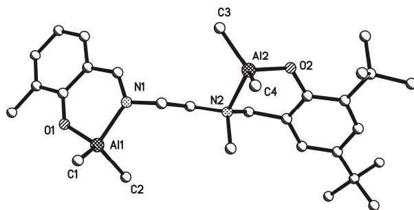
Fig. 2 Molecular structure of \text{Al}_2(3)\text{Me}_4 . Selected bond lengths ( \text{\AA} ) and angles ( ^{\circ} ) are Al(1)-O(1) 1.7750(13), Al(1)-C(2) 1.952(2), Al(1)-N(1) 1.9613(15), Al(1)-C(1) 1.9624(19), Al(2)-O(2) 1.7638(13), Al(2)-C(3) 1.950(2), Al(2)-C(4) 1.957(2), Al(2)-N(2) 2.0577(15), O(1)-Al(1)-C(2) 114.01(8) , O(1)-Al(1)-N(1) 95.00(6) , C(2)-Al(1)-N(1) 105.89(8) , O(1)-Al(1)-C(1) 111.74(7) , C(2)-Al(1)-C(1) 118.11(9) , N(1)-Al(1)-C(1) 109.22(8) .
