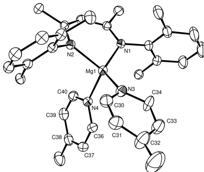
Figure 3: ORTEP representation (25% probability ellipsoids) of the X-ray structure of compound 6 . Hydrogen atoms and iso -propyl methyl groups are deleted for clarity.
