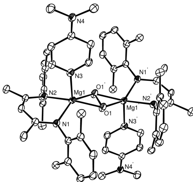
Figure 6: ORTEP representation (25% probability ellipsoids) of the X-ray structure of compound 12 . Hydrogen atoms and iso -propyl methyl groups are deleted for clarity. Symmetry transformations used to generate equivalent atoms: #1 -x+2,-y,-z.
