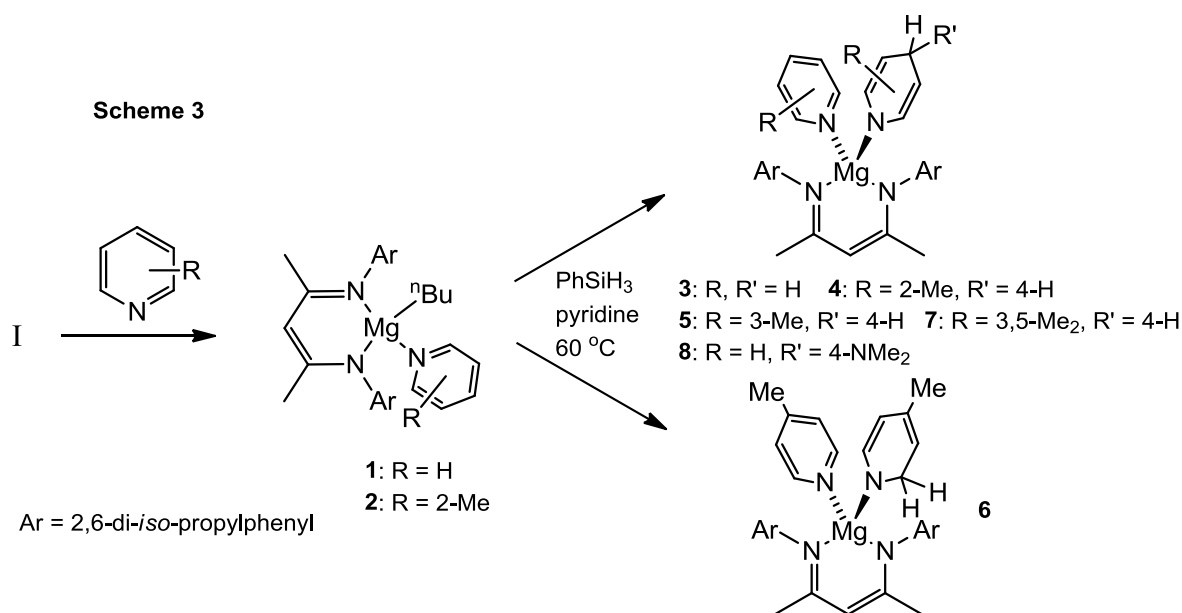
Scheme 3: Dearomatisation of pyridine derivatives by 1 and PhSiH 3 .
