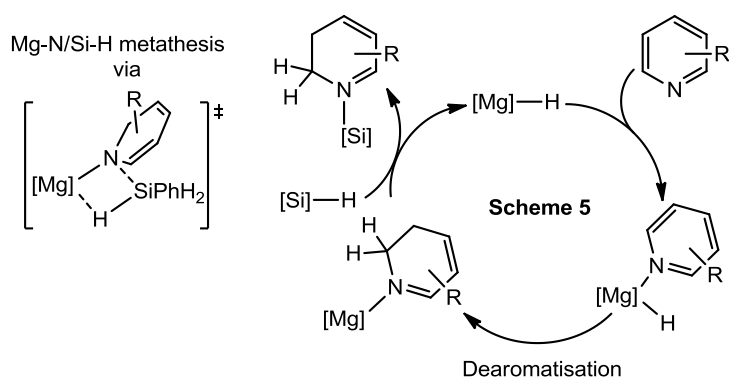
Scheme 5: Proposed mechanism for the magnesium-catalysed hydrosilylation of pyridine derivatives.
