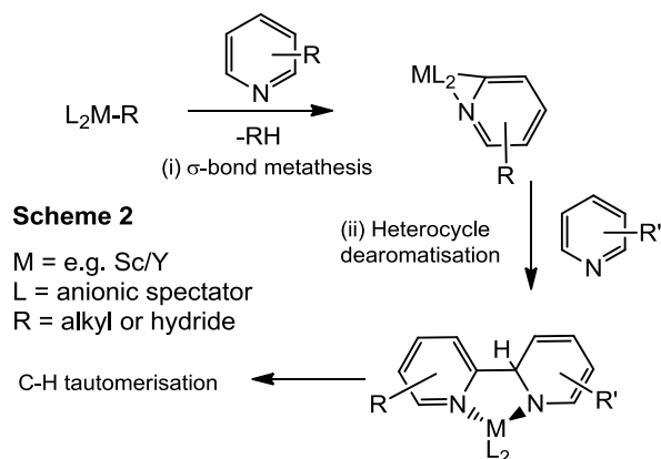
Scheme 2: Group 3-catalysed pyridine ortho -CH activation and dearomatisation/coupling. 10
