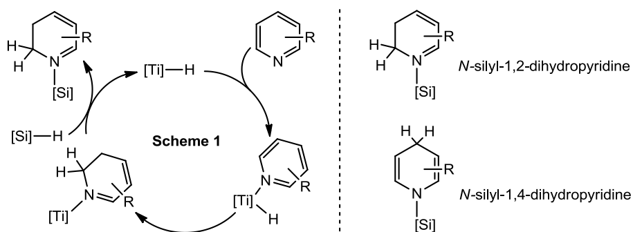
Scheme 1: Proposed mechanism for the titanocene-catalysed hydrosilylation of pyridine. 5
