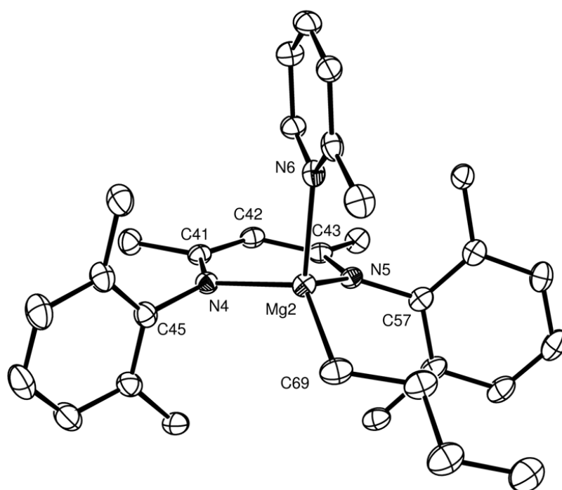
Figure 1: ORTEP representation (25% probability ellipsoids) of the X-ray structure of compound 2 . Hydrogen atoms and iso -propyl methyl groups are deleted for clarity.
