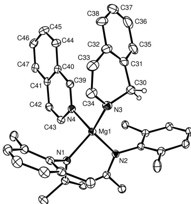
Figure 4: ORTEP representation (25% probability ellipsoids) of the X-ray structure of compound 10 . Hydrogen atoms except those attached to C(30) and iso -propyl methyl groups are deleted for clarity.
