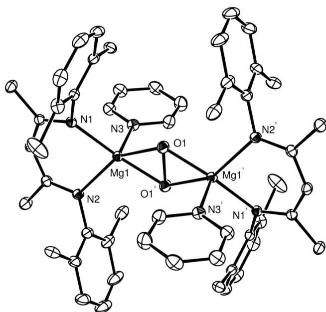
Figure 5: ORTEP representation (25% probability ellipsoids) of the X-ray structure of compound 11 . Hydrogen atoms and iso -propyl methyl groups are deleted for clarity. Symmetry transformations used to generate equivalent atoms: #1 -x+1, -y, -z+2.
