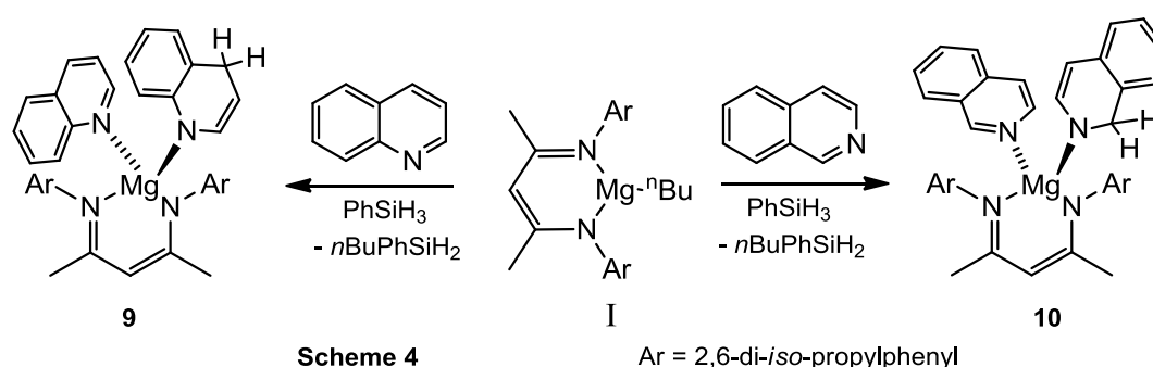
Scheme 4: Dearomatisation of quinoline derivatives by 1 and PhSiH 3 .
