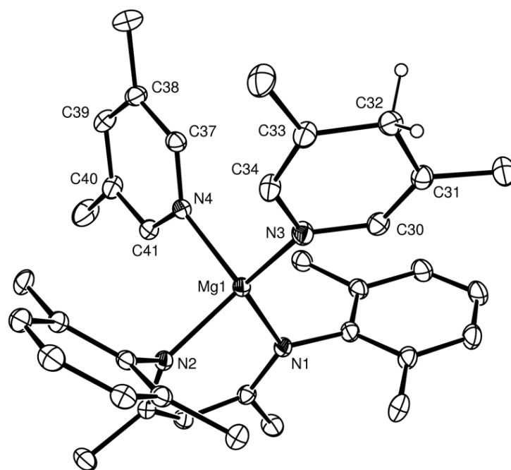
Figure 2: ORTEP representation (25% probability ellipsoids) of the X-ray structure of compound 7 . Hydrogen atoms except those attached to C(32) and iso -propyl methyl groups are deleted for clarity.
