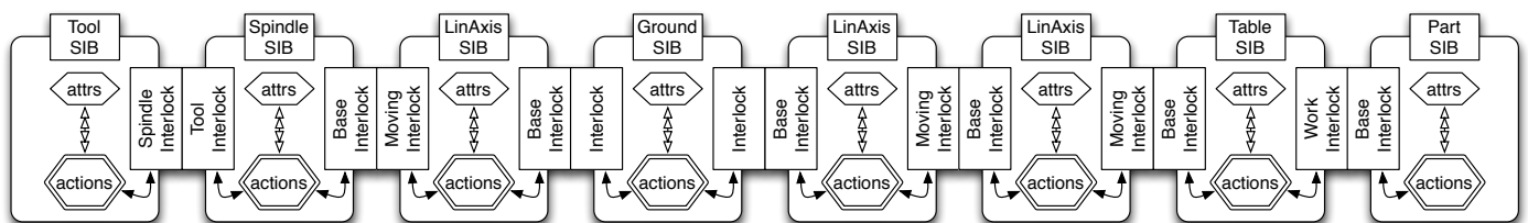
Figure 7. Simplified SIB model of a 3-axis vertical machining center
