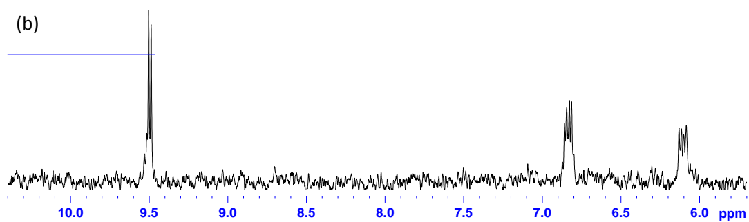
Fig. S3 (a) 1 H- 1 H COSY and (b) 1D 1 H TOCSY (selectively excited at \delta 9.50 ppm) NMR spectra, taken at 24 hours into the oxidation of RME at 150 °C, showing the identity of a trans unsaturated aldehyde. Only the region between \delta 10.4 and \delta 5.7 ppm is shown.
