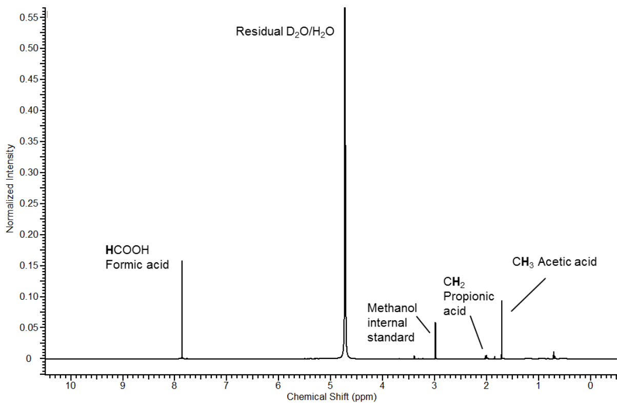
Fig. S4 ^1\text{H} NMR spectra of the \text{D}_2\text{O} trap, collected after 24 hours for the oxidation of RME at 150\text{ }^\circ\text{C}
