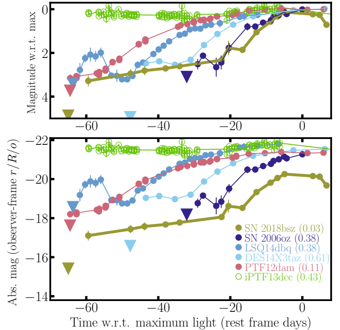
Fig. 7. Comparison of the pre-maximum light curve of SN 2018bsz to those of SLSNe-I from the literature showing clear bumps before the main rise to maximum (iPTF13dcc is shown in open circles as its form is clearly distinct from the events). Next to each SLSN name in parenthesis we give the object redshift (in the bottom panel ). Non-detection upper limits are indicated by upside down triangles. Top : light-curves normalised to maximum-light magnitude. Bottom : absolute magnitude light curves with respect to maximum light. SN 2018bsz is in the ATLAS o band, while all other comparison SNe are in observed R or r band. Given the range of redshifts of the SLSN comparison sample, these observed bands equate to different rest frame wavelengths. However, given the lack of a) multi-band photometry (to enable rest-frame band comparison) and b) spectra of SLSNe-I during these epochs (to allow for valid K -corrections) we prefer to plot the data in its “raw” form. Colour effects may complicate the direct comparison of these light curves.
