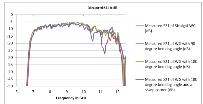
Fig.9. Comparison of measured S21 of knitted waveguide under different E-plane conditions
