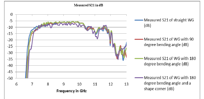
Fig. 5. Comparison of measured S21 of knitted waveguide under different H-plane conditions
