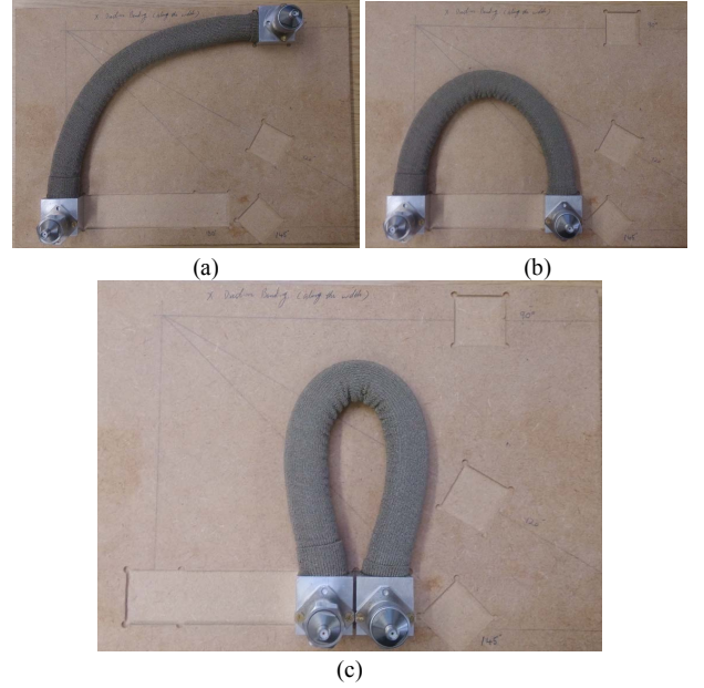
Fig. 4. Knitted waveguide under principle H-plane bending. (a): Bending angle: 90 degree, (b): Bending angle: 180 degree, (c): Bending angle: 180 degree with a sharp corner
