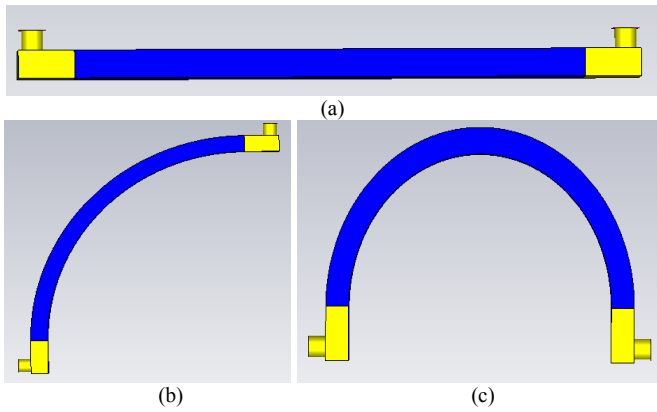
Fig.6. Waveguide under different conditions in simulation (a): Straight, (b): Bending angle 90 degree, (c): Bending angle 180 degree
