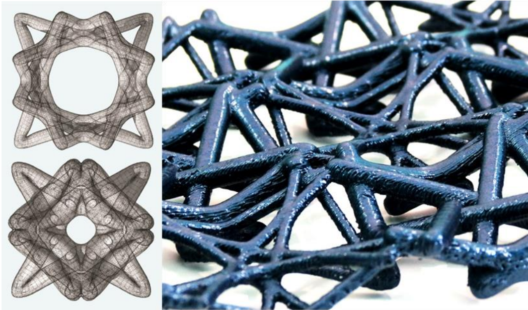
Figure 3: LEFT: Parametric Variation of parts through aperture and thickness. RIGHT: 3D printed ABS Mashrabiya prototype finished in automotive paint to enable exterior installation.
