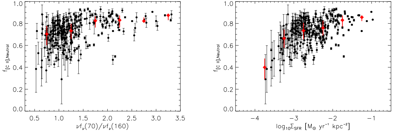
Figure 3. The fraction of [C II] emission that originates in the neutral phase, assuming a solar C/N ratio, plotted as a function of the far-IR color (left) and the star formation rate surface density (right). Data binned to equal intervals are plotted as red diamonds, with error bars denoting the 25-75% percentile ranges in each bin. While there are weak correlations there is also significant scatter, particularly in gas described by a cool dust temperature.
