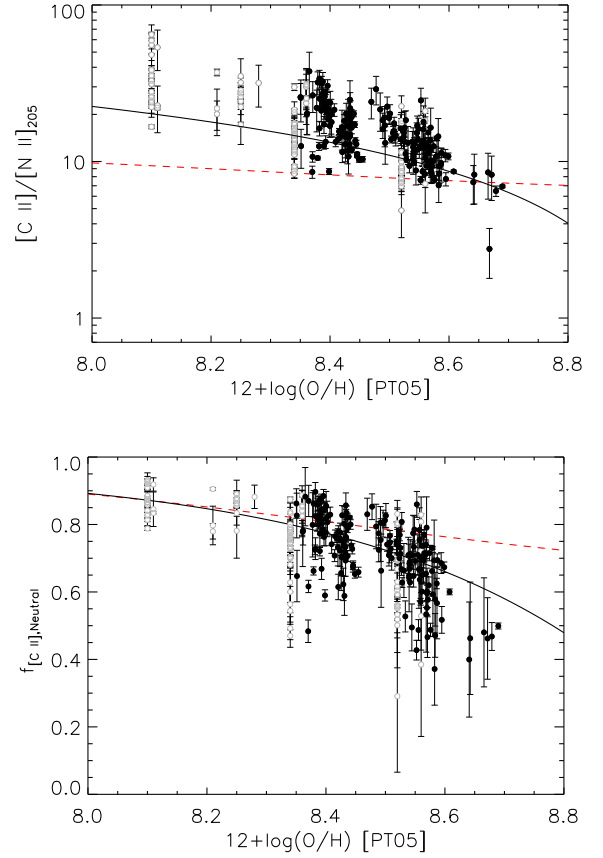
Figure 4. Top: The ratio of [\text{C II}]/[\text{N II}] 205 \mu\text{m} as a function of gas-phase oxygen abundance. Bottom: The fraction of [\text{C II}] emission originating in the neutral phase plotted as a function of the metallicity, assuming \text{C}/\text{N}_{\odot} . Regions in galaxies for which Moustakas et al. (2010) determined a gradient are plotted as filled points while open points indicate global O/H measurements. The black lines represent a fit to f_{[\text{C II}],\text{Neutral}} and the linear O/H ratio while the dashed red lines show the arbitrarily normalized, modest trends expected if the [\text{C II}] neutral fraction were in fact fixed, and changes in [\text{C II}]/[\text{N II}] 205 \mu\text{m} and f_{[\text{C II}],\text{Neutral}} were driven solely by underlying C/N variation with 12+\log(\text{O}/\text{H}) as expressed in Eq. 2. The O/H abundance is on the scale of Pilyugin & Thuan (2005).
