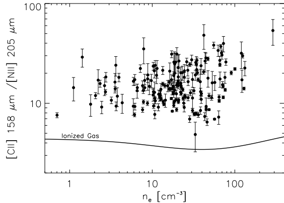
Figure 2. The ratio of total [C II]/[N II] 205 \mu\text{m} as a function of density. Data show the line ratio observed in the bulk ISM of nearby galaxies, whereas the line denotes the theoretical predictions for ionized gas. The fact that all ratios are elevated above this prediction indicates that non-ionized gas makes a significant contribution to the [C II] emission. The flatness of the predicted contribution from ionized gas demonstrates how can avoid the dependence of [C II]/[N II] on density.
