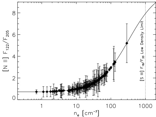
Figure 1. The observed ratio of the two far-IR [N II] lines plotted as a function of density, derived from the theoretical line ratio, shown as the solid line. While the Herschel data are consistent with [N II] originating in the low-density regime, as defined by [S III] emission ( n \leq 1000 ), N^+ ions clearly exist in a range of low-density environments, affecting the predicted ratio of [C II]/[N II] 122 \mu\text{m} . This means that [C II]/[N II] 122 \mu\text{m} is an unreliable tracer of ionized [C II] and observations of the [N II] 205 \mu\text{m} is required to trace the contributions to [C II] from ionized gas.
