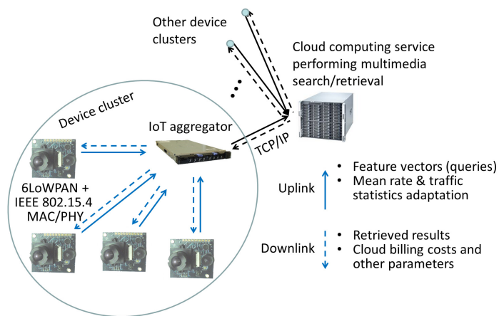
Figure 1. System hierarchy for a media search application within an IoT context. Low-power devices send query data to an IoT aggregator using low-power protocols for the physical, medium access control and network layer, such as IEEE 802.15.4 MAC/PHY and 6LoWPAN. The IoT aggregator sends aggregated query volumes to the cloud-computing service using TCP/IP.
