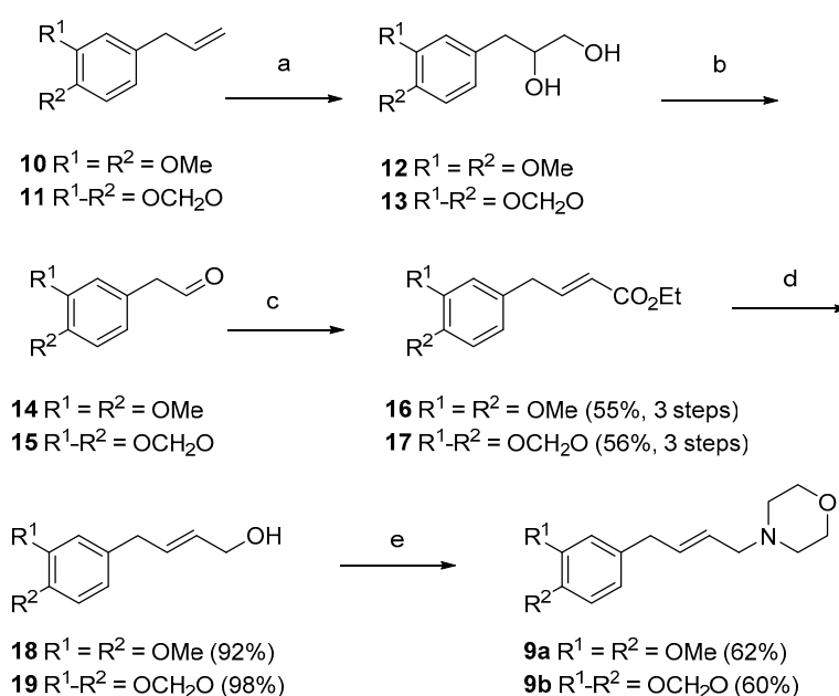
Scheme 1. (a) OsO 4 (0.1–0.3 mol%), N -methylmorpholine- N -oxide (3 eq.), t BuOH/H 2 O (1:1), 4 days; (b) NaIO 4 (1.2 eq.), MeOH/H 2 O (3:1), 0.5–2 h; (c) Ph 3 PCHCO 2 Et (1.1 eq.), CH 2 Cl 2 , 16 h; (d) 18 : DIBAL-H (3 eq.), CH 2 Cl 2 , –78 °C, 10 min, 19 : DIBAL-H (2.2 eq.), toluene, –10 °C, 10 min; (e) Et 3 N (3 eq.), MsCl (1.2 eq.), morpholine (1.5 eq.), CH 2 Cl 2 , 0 °C, 2–18 h.
