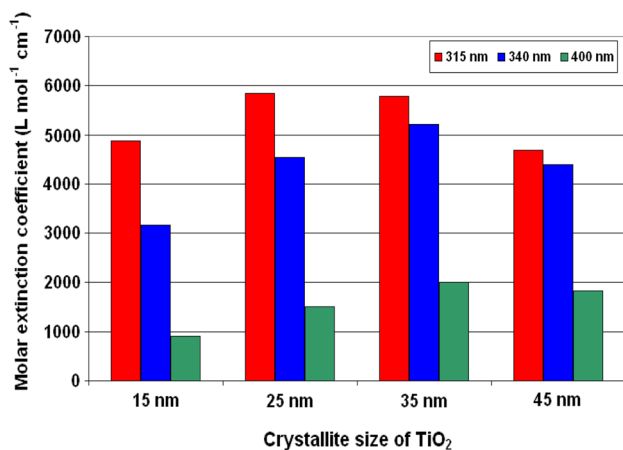
Fig. 5 Molar extinction coefficient for TiO 2 of various crystallite sizes at various wavelengths. Thin films of isocyanate acrylic containing TiO 2 at 2% on weight of resin solids
