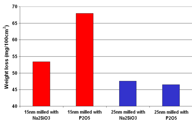
Fig.9 Weight loss of isocyanate acrylic coatings containing UV blocker products surface treated with SiO 2 /Al 2 O 3 /P 2 O 5 after 2332 h Atlas exposure
