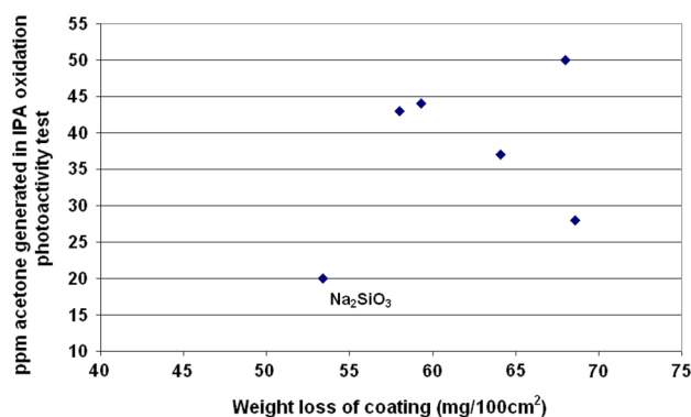
Fig. 7 Parts per million (ppm) acetone generated in the IPA oxidation test versus weight loss of isocyanate acrylic coating containing the UV blockers
