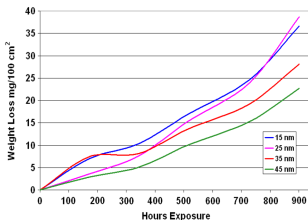
Fig. 6 Weight loss of an isocyanate acrylic coating containing TiO 2 of various crystallite sizes
