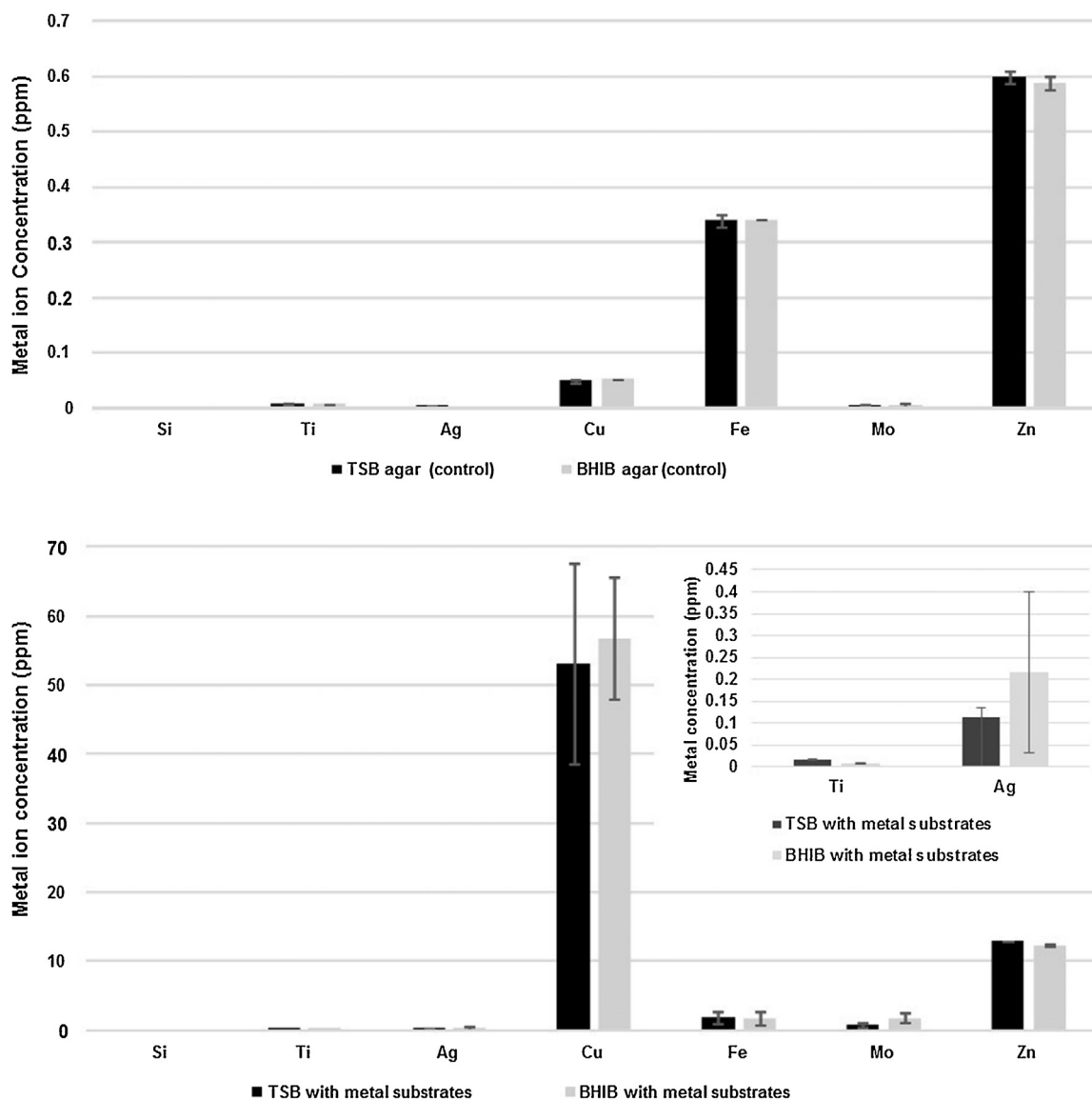
Fig. 1 – Metal ion concentrations in (A) TSB and BHIB control media prior to incubation with substrata, and (B) in TSB and BHIB media post incubation with coated substrates demonstrating Cu displayed the greatest leaching rate when incubated in the media (data is presented as mean ± SD). Note the difference on the y axis in A and B.
