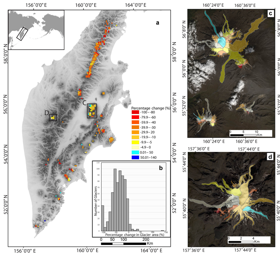
Figure 4. Percentage change in glacier surface area across the Kamchatka Peninsula between 2000 and 2014. (a) Mean values shown for 5 × 5 km grid cells. (b) Values for individual glaciers shown as a frequency distribution. (c) Values for individual glaciers in the Klyuchevskaya volcanic group. (d) Values for individual glaciers on the slopes of Ichinsky Volcano. In both (c) and (d), the colour scheme from (a) is used.
