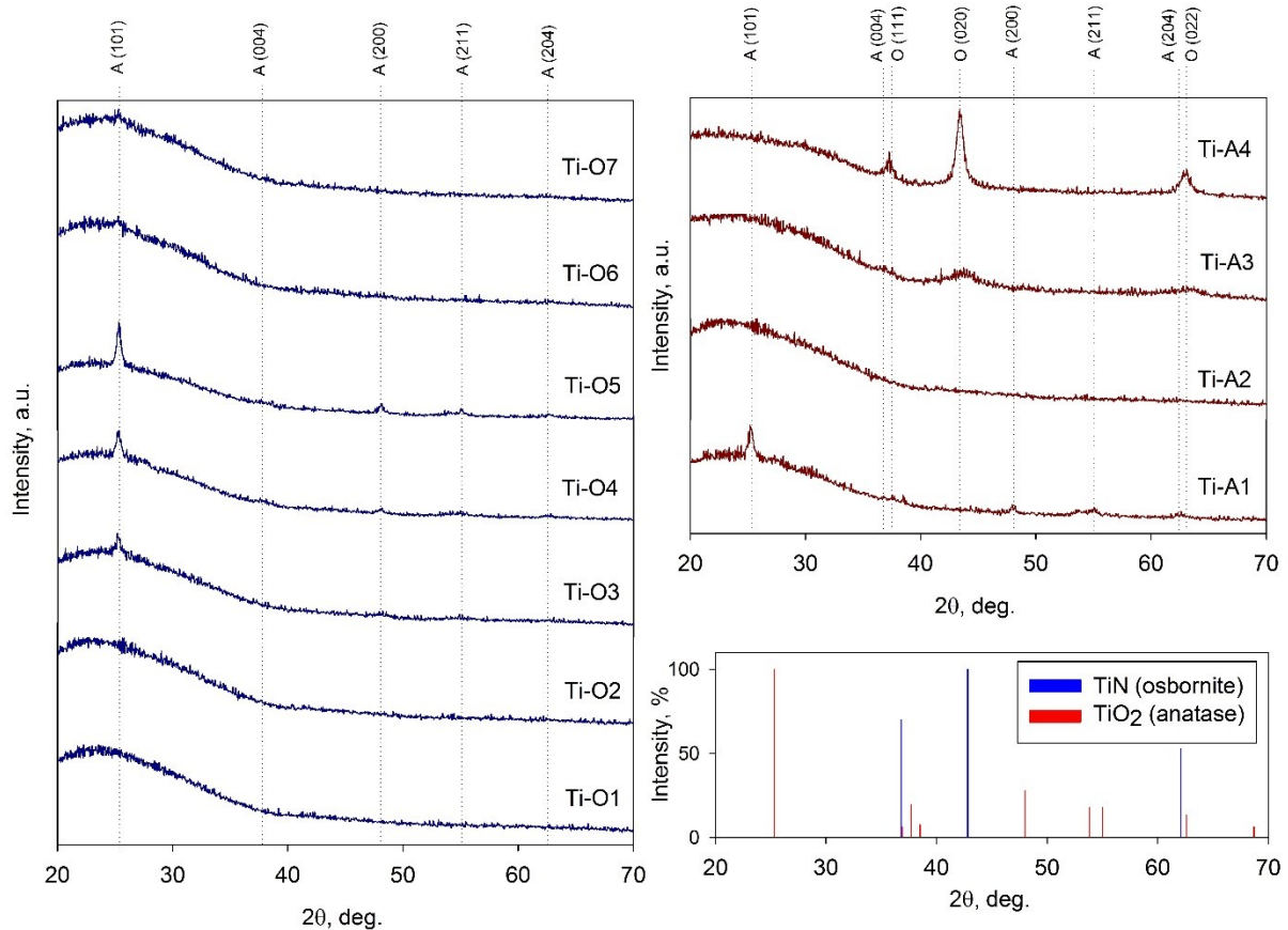
Figure 3. XRD diffraction patterns of the coatings: deposited using oxygen as reactive gas (left, blue); using air as reactive gas (top right, red); crystallographic patterns (bottom right)
