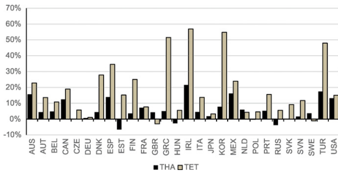
Fig. 3. TET and THA: percentage variation between the years 1995 and 2007.
