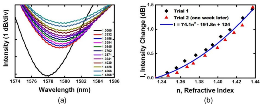
Fig. 5. (a) Output spectra of the sensing element, focusing particularly on the variation of the selected interference dip at 1577.68 nm when the sensing element was immersed in various solutions of different RIs. (b) Plot of the change in intensity of the interference dip shown in (a) against the RI of the various solutions for two separate trials (diamonds and triangles) conducted one week apart. The nonlinear behavior of the sensing element to variations in RI is illustrated by the single fitting curve (solid line).
