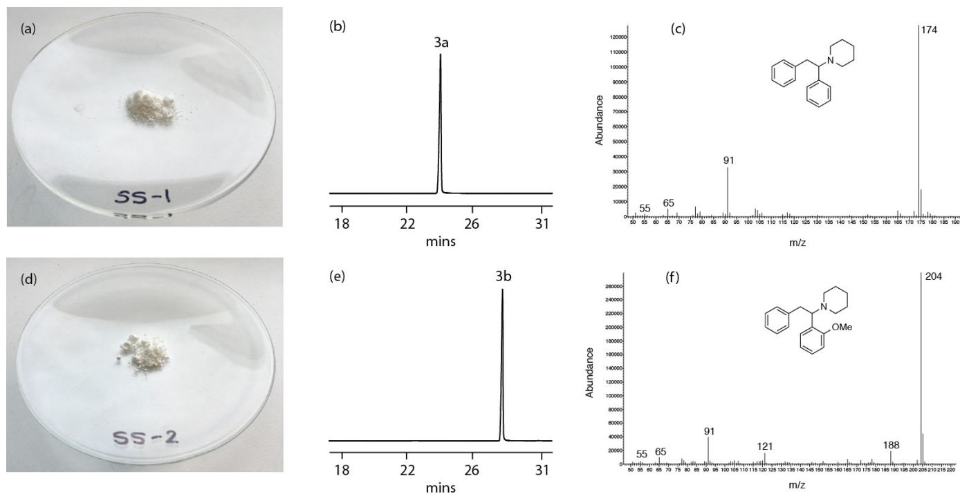
Figure 4. Qualitative GC–MS analysis of the diphenidine (SS-1, 0.1 mg mL -1 in methanol) and methoxphenidine (SS-2, 0.1 mg mL -1 in methanol) products: (a) diphenidine sample (1 g, SS-1) obtained from “Buy Research Chemicals UK” ( http://www.brc-chemicals.com ); (b) GC chromatogram for SS-1; (c) EI-MS spectrum (+ve ion mode) of peak ( t_R = 23.72 min) corresponding to diphenidine ( 3a , [M+H]^+ = 174 , base peak); (d) methoxphenidine sample (1 g, SS-2) obtained from “Buy Research Chemicals UK” ( http://www.brc-chemicals.com ); (e) GC chromatogram for SS-2; (f) EI-MS spectrum (+ve ion mode) of peak ( t_R = 28.06 min) corresponding to 2-methoxphenidine ( 3b , [M+H]^+ = 204 , base peak). See Materials and Methods (Section 2.4 and 2.6) for experimental details.
