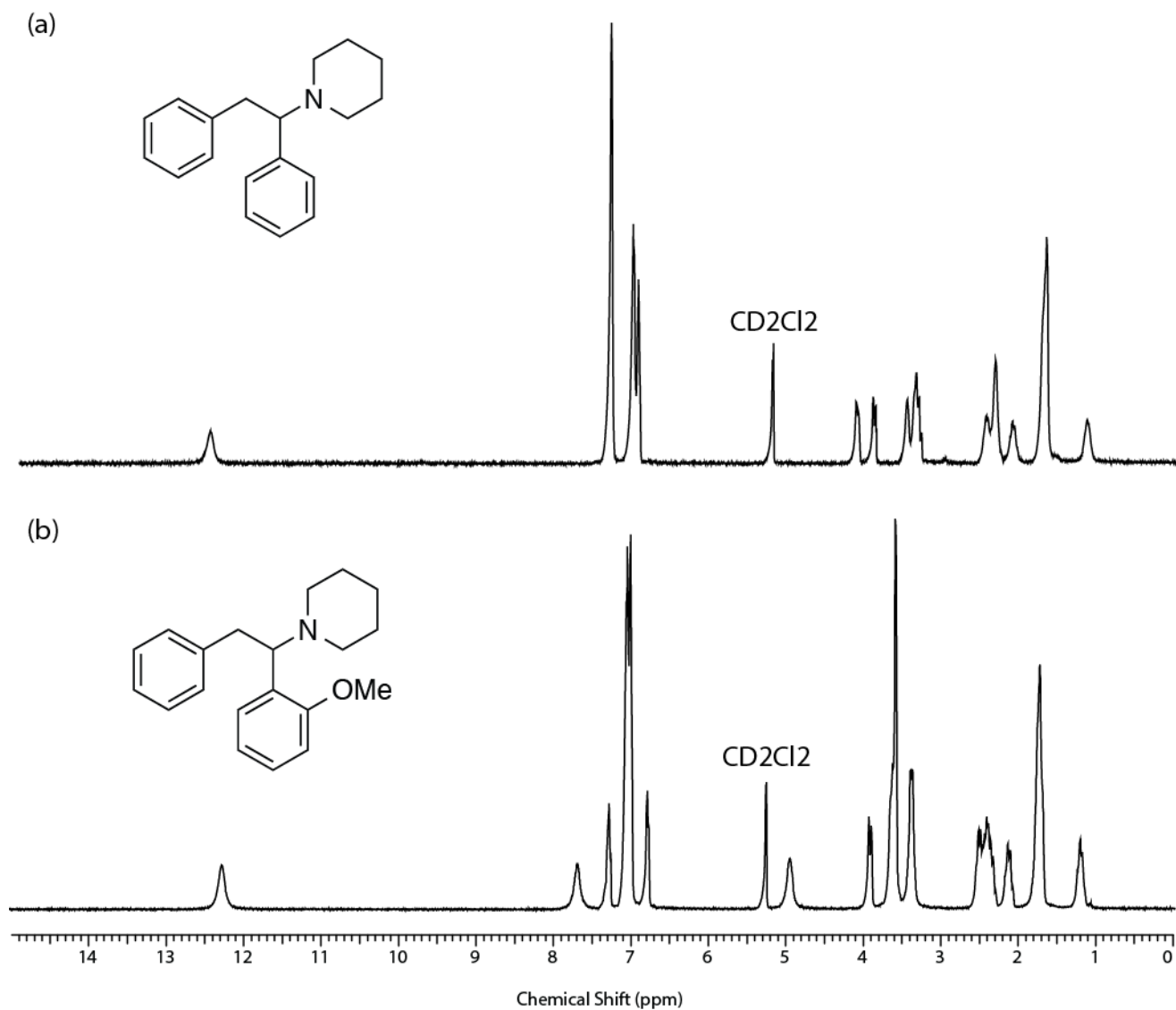
Figure 5. ^1\text{H-NMR} (400 MHz, \text{CD}_2\text{Cl}_2 ) analysis of (a) diphenidine (SS-1, 10 mg/600 \mu\text{L} ) and (b) methoxphenidine (SS-2, 10 mg/600 \mu\text{L} ) products obtained from “Buy Research Chemicals UK” ( http://www.brc-chemicals.com ).
