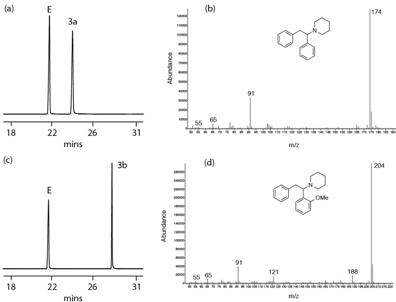
Figure 6. Quantitative GC–MS analysis of the diphenidine (SS-1, 0.1 mg mL -1 in methanol containing 0.1 mg mL -1 eicosane, E) and methoxphenidine (SS-2, 0.1 mg mL -1 in methanol containing 0.1 mg mL -1 eicosane, E) products: (a) GC chromatogram for SS-1; (b) EI-MS spectrum (+ve ion mode) of peak ( t_R = 23.72 min) corresponding to diphenidine ( 3a , [M+H]^+ = 174 , base peak); (c) GC chromatogram for SS-2; (d) EI-MS spectrum (+ve ion mode) of peak ( t_R = 28.06 min) corresponding to 2-methoxphenidine ( 3b , [M+H]^+ = 204 , base peak). See Materials and Methods (Section 2.4 and 2.7) for experimental details. NB. t_R (eicosane) = 21.55 min.
