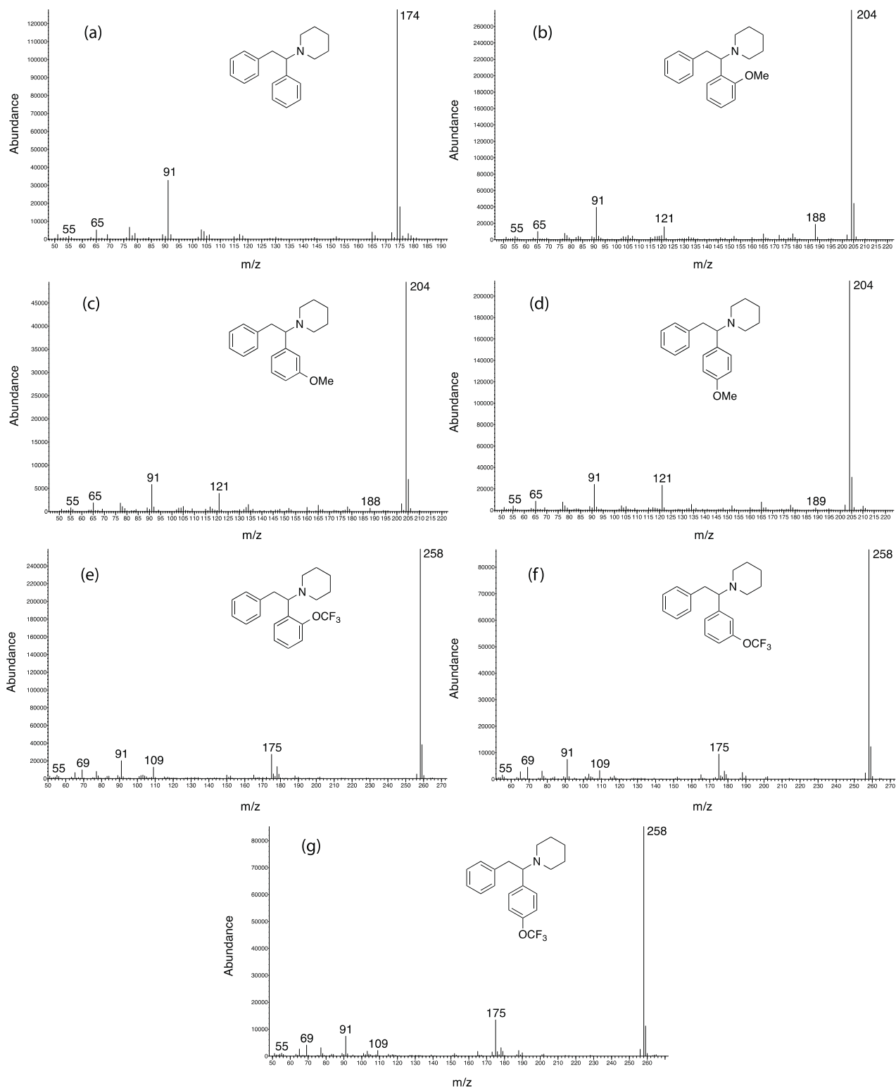
Figure 2. EI-MS spectra of (a) diphenidine ( 3a ) and its substituted derivatives (b) 2-methoxyphenidine (2-MXP, 3b ); (c) 3-methoxyphenidine (3-MXP, 3c ); (d) 4-methoxyphenidine (4-MXP, 3d ); (e) 2-trifluoromethoxyphenidine (2-TFMXP, 3e ); (f) 3-trifluoromethoxyphenidine (3-TFMXP, 3f ) and (g) 4-trifluoromethoxyphenidine (4-TFMXP, 3g ).
