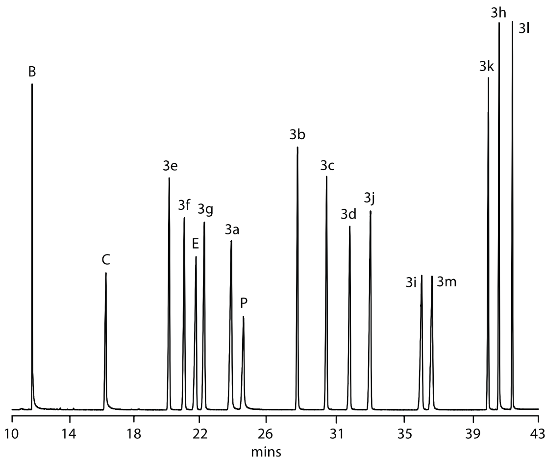
Figure 1. Exemplar chromatogram demonstrating separation of all thirteen substituted diphenidines and relevant adulterants: benzocaine (B); caffeine (C); 2-trifluoromethoxyphenidine (2-TFMXP, 3e ); 3-trifluoromethoxyphenidine (3-TFMXP, 3f ); eicosane (internal standard, E); 4-trifluoromethoxyphenidine (4-TFMXP, 3g ); diphenidine ( 3a ); procaine (P); 2-methoxyphenidine (2-MXP, 3b ); 3-methoxyphenidine (3-MXP, 3c ); 4-methoxyphenidine (4-MXP, 3d ); 3,4-(methylenedioxy)diphenidine (3,4-MDDP, 3j ); 2,3-(methylenedioxy)diphenidine (2,3-MDDP, 3i ); IAS-013 ( 3m ); 1-naphthenidine (1-NPD, 3k ); mescphenidine (3,4,5-TMXP, 3h ) and 2-naphthenidine (2-NPD, 3l ) [Underlined compounds are common adulterants]. See Materials and Methods (Section 2.4) for experimental details.
