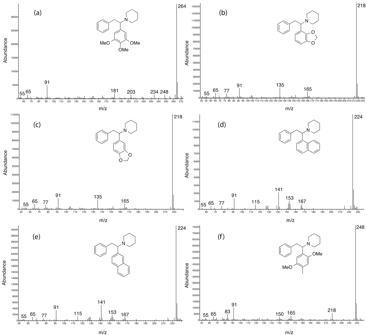
Figure 3. EI-MS spectra of (a) mesphenidine (3,4,5-TMXP, 3h ); (b) 2,3-(methylenedioxy)diphenidine (2,3-MDDP, 3i ); (c) 3,4-(methylenedioxy)diphenidine (3,4-MDDP, 3j ); (d) 1-naphthenidine (1-NPD, 3k ); (e) 2-naphthenidine (2-NPD, 3l ); (f) IAS-013 ( 3m ).
