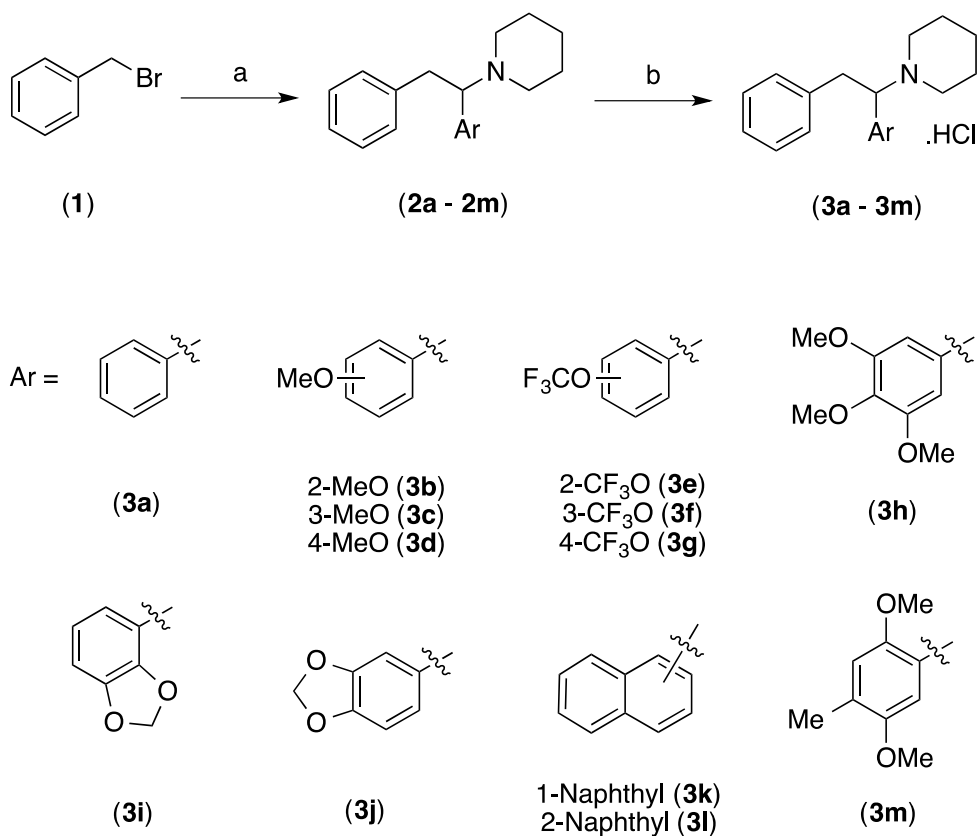
Scheme 1. Reagents and Conditions: (a) Zn/TFA/ArCHO/piperidine; (b) HCl (4M solution in dioxane)/Et 2 O (21 – 77% yield). See Materials and Methods (Section 2.1) for experimental details.
