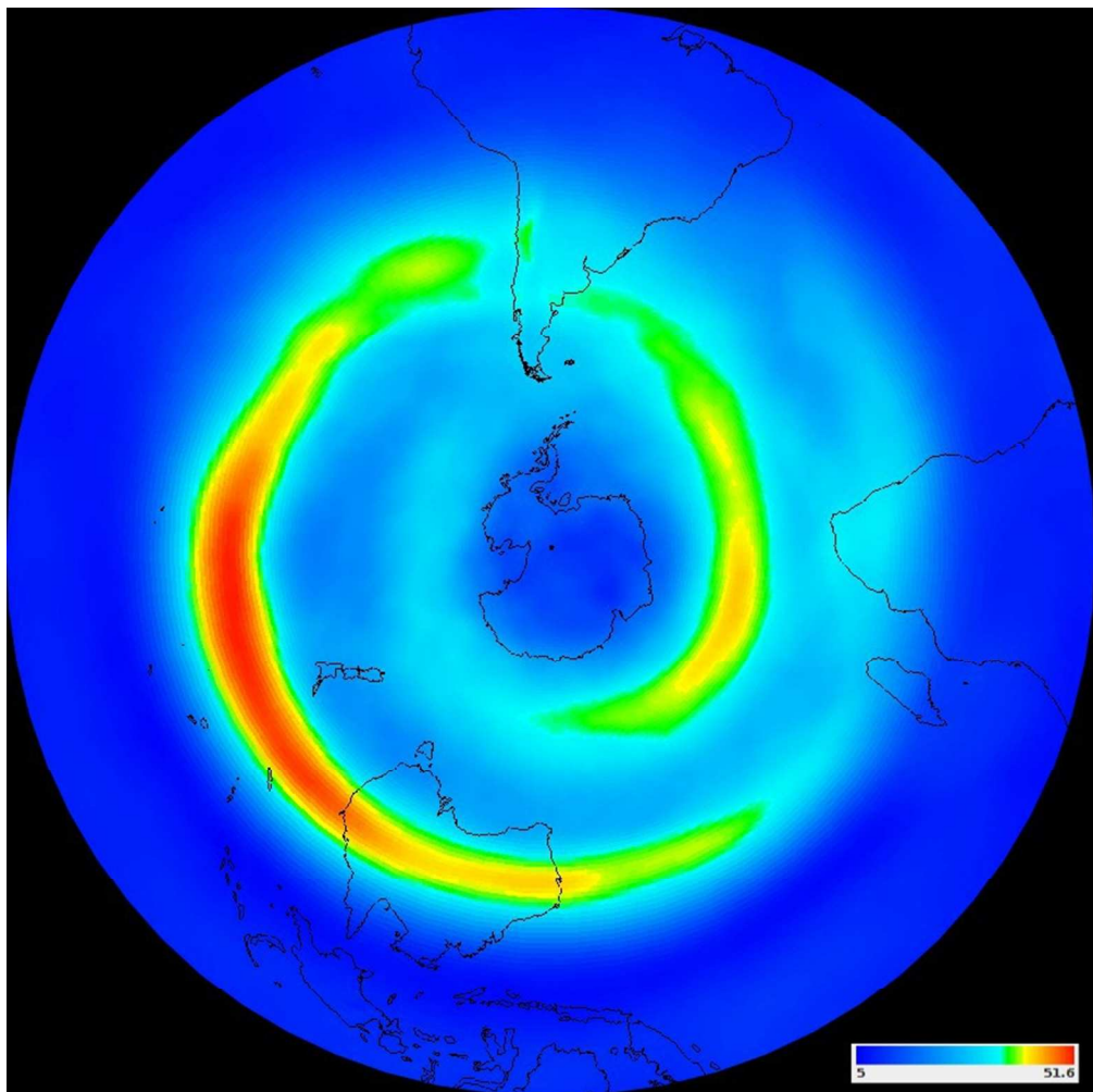
JJA 2015 mean wind velocity at 300hPa.
