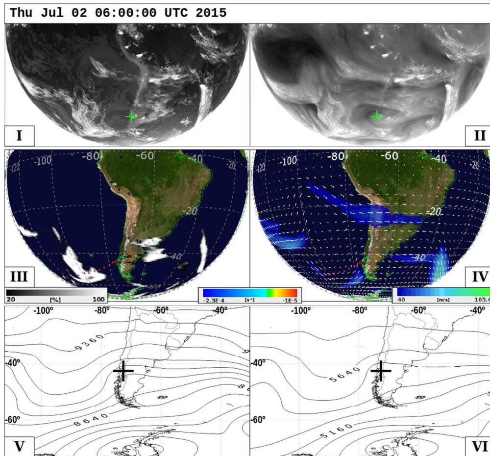
Validation Event 2 June 27th -July 11th, 2015. Same as Fig. 11 but for validation event 2. b. July 2nd, 2015 at 06:00 UTC
