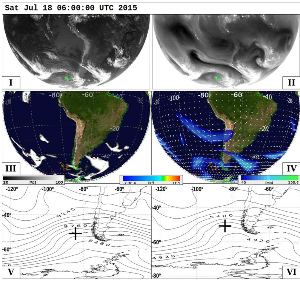
Validation Event 3 July 10th- July 24th, 2015. Same as Fig. 11 but for validation event 3. a. July 18th, 2015, at 06:00 UTC,
