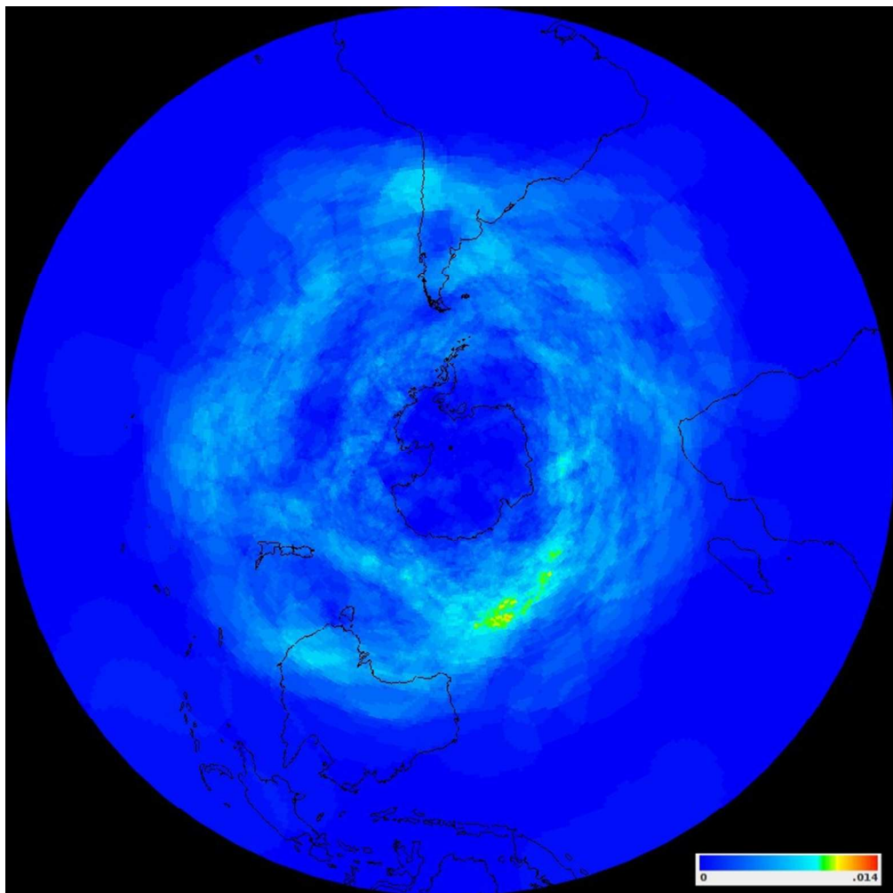
JJA 2015 Intermediate cyclone event densities over the SH: c. middle to upper troposphere events.
