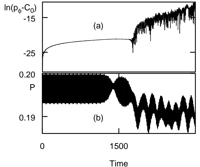
FIG. 6. N = 144 , \tau = 233/144 , \lambda = 0.05 , P_0 = 0.20 . (a) Time evolution of \log(p_\phi - C_0) . (b) CM momentum P . Note that the CM momentum has begun its decay before the deviation of p_\phi from its constant value occurs.
