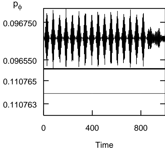
FIG. 3. Behavior of p_\phi for the parameters of the model as described in Fig. 2. (a) Incommensurate case: the GAM is constant within numerical precision. (b) Commensurate case: the GAM is not conserved. Note the change of scale going from panel (a) to panel (b).
