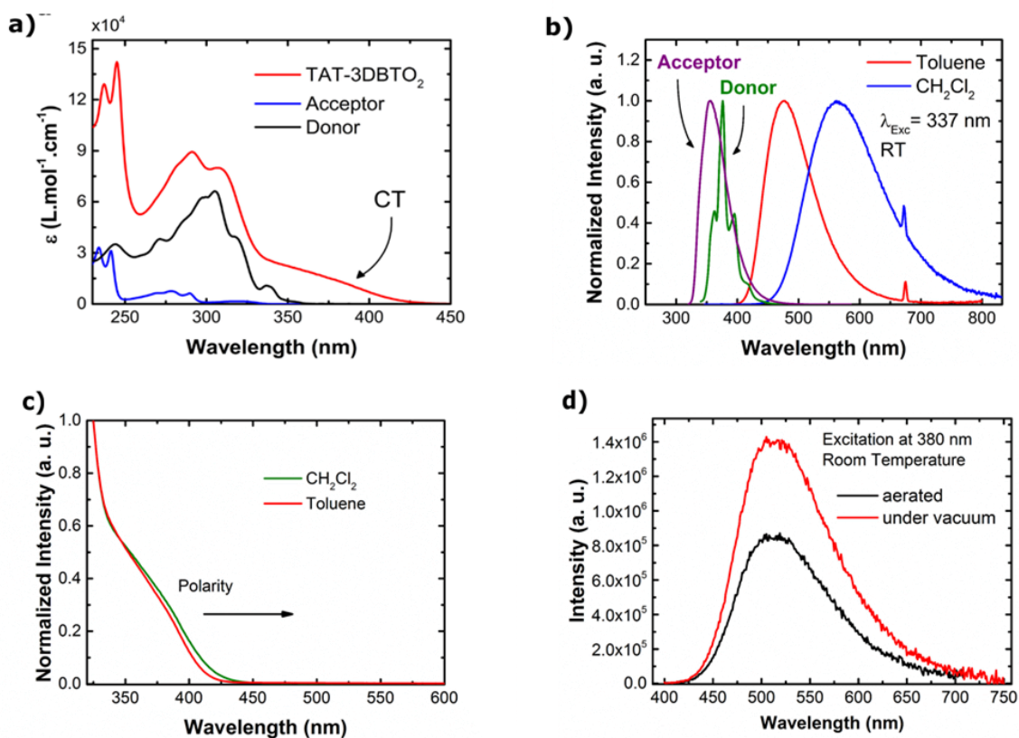
Figure 55 a) Extinction coefficient spectra of the acceptor (A), donor (D), and TAT-3DBTO 2 molecules, all diluted in dichloromethane (CH 2 Cl 2 ) solvent. b) Normalized photoluminescence (PL) spectra of acceptor (data taken from ref 13 ), donor, and TAT-3DBTO 2 molecules. D and A are diluted in toluene solvent, TAT-3DBTO 2 diluted in toluene and CH 2 Cl 2 . c) Absorption spectra of TAT-3DBTO 2 in CH 2 Cl 2 and toluene. d) PL spectra of TAT-3DBTO 2 :BCPO film under vacuum and in air.
