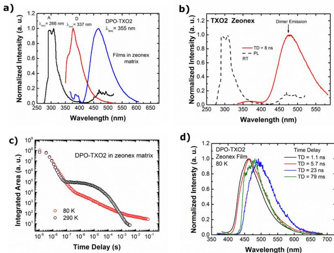
Figure 23 a) Normalized photoluminescence (PL) spectra of acceptor (A), donor (D), and DPO-TXO2 molecules, all dispersed in zeonex matrix. b) Time resolved fluorescence emission of A together with its PL spectrum. c) Time resolved fluorescence decay of DPO-TXO2 in zeonex matrix. The curves were obtained with 355 nm excitation. d) Time resolved normalized emission spectra in the entire region of analyses at 80K.
