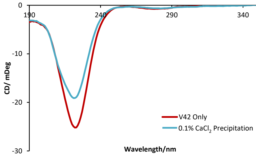
Figure 60: CD spectra of V42 incubated at 20 °C under nil detergent, control conditions (MEA buffer at pH8, red) and in 0.1% LAS, with surfactant removal by CaCl 2 precipitation and centrifugation (Blue).
