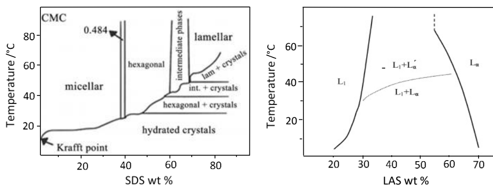
Figure 5: Phase Diagrams of SDS (left) and LAS (right) in water at various temperatures and concentrations. Figures reproduced with permission from Rossi et al 42 and Stewart et al 43 .
