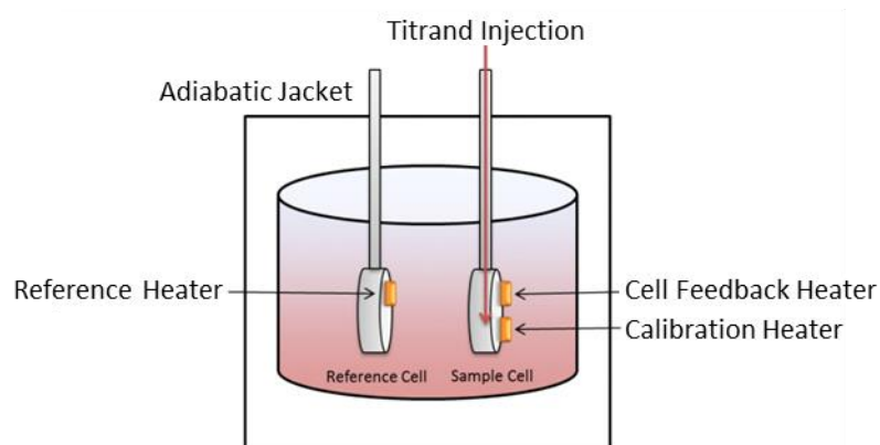
Figure 13: Schematic of Isothermal Scanning Calorimetry.
