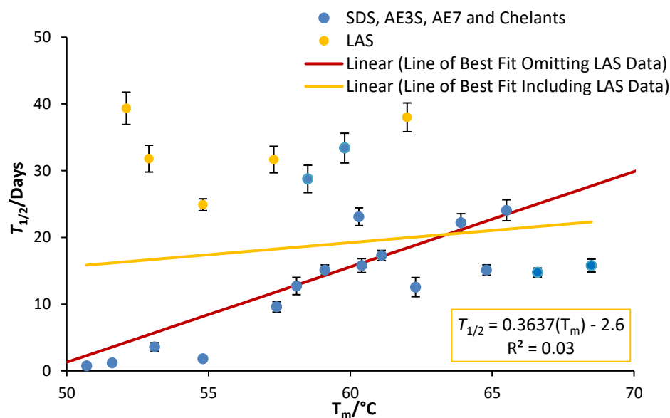
Figure 112: Plot of V42 T_{1/2} as a function of T_m values for V42 determined by CD. Outlying LAS data is included in orange. Data points excluded from calculation of best fit line are represented by unfilled circles.
