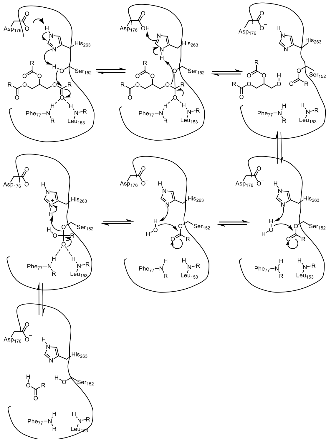
Figure 4: Hydrolysis of a triglyceride by lipase. 31-33
