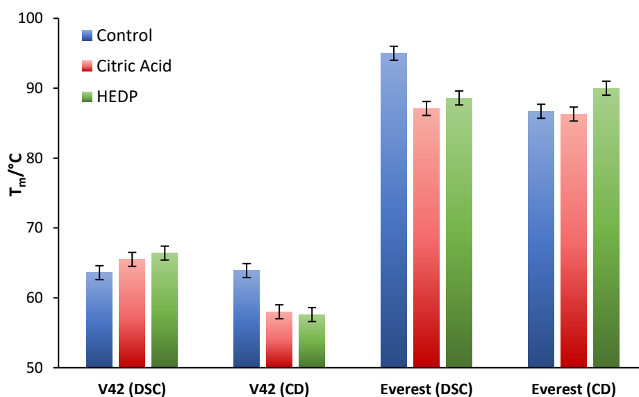
Figure 45: Comparison of T_{max} values obtained by CD and DSC for Everest and V42 in the presence of HEDP and Citric Acid.
