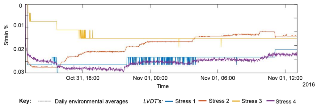
Figure 5.11: Monitoring strain data a) Strain response for each of the four stressed siltstone samples within the laboratory experiments (Table 1). An increase in strain values reflects compression of the sample, while decreases in strain values reflect expansion of sample. Rebound occurs at the end of the experiment for all samples once the constant uniaxial compressive stress is removed. b) First 24 hours of experiment, displaying an initial compression for all samples, followed by either further compression as is the case for Stress 3, or expansion as seen for Stress 1, 2 and 4.
