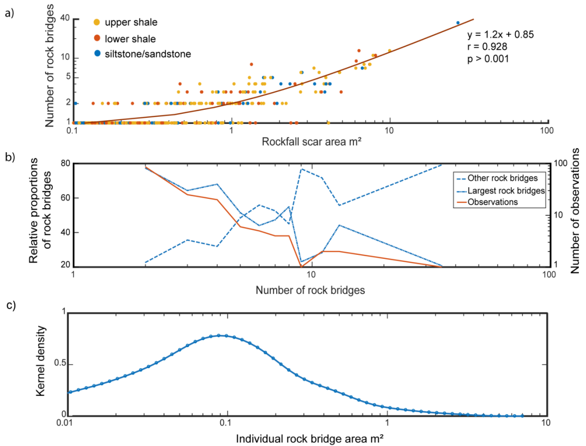
Figure 3.12: Rock bridge distribution within each rockfall scar. a) Scatter plot displaying a positive linear trend between number of rock bridges per scar and rockfall scar area. b) Mean values of the relative proportion of the largest rock bridge within an individual scar compared with the proportion of all other rock bridges within an individual scar. For example, if a rockfall scar contains two rock bridges, the largest accounts for 80% of rock bridge area while the other accounts for only 20 %. The number of observations for the calculation of mean values is plotted on the right axis and decreases with increasing rock bridges. c) Kernel density plot of individual rock bridge area distribution, displaying that most rock bridges are 0.1 m 2 .
