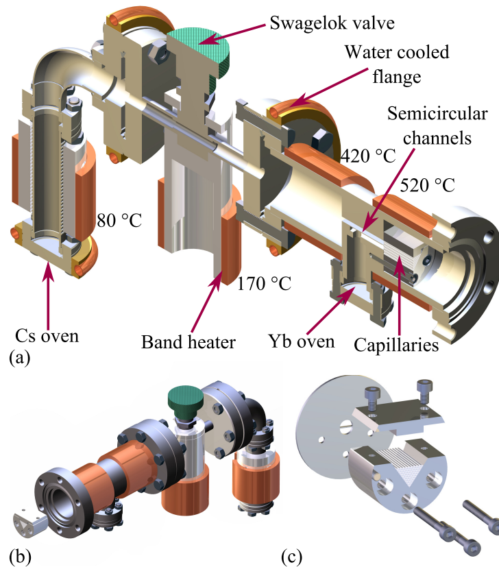
Figure 3.3: (a) A cutaway schematic of the dual species oven showing the paths of the two species through the oven. The nozzle heaters are shown as copper bands and the water cooling as copper tubes. The temperatures displayed are the nozzle heater set points, the Yb chamber is typically measured to be at 485 °C. (b) Rendering of the oven with the capillary clamp shown outside the oven for detail. (c) Exploded view of the capillary array and the wire-eroded semicircular channels that the array is clamped over within the oven.
