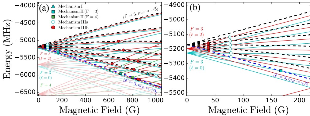
Figure 9.2: (a) Level crossing diagram for ^{133}\text{Cs}^{173}\text{Yb} . Binding energy from centre of weight of the hyperfine structure versus magnetic field strength. The dashed black lines are atomic levels, the solid lines are molecular levels, with cyan corresponding to the \ell = 0 levels of the lower ( F=3 ) hyperfine manifold, red the \ell = 2 levels of this manifold and green corresponding to the upper ( F=4 ) hyperfine manifold ( \ell = 0 levels). The atomic level of |F = 3, m_F = +3\rangle is highlighted in blue. Markers denote level crossings that produce resonances, the relevant coupling is indicated by the marker shape: triangles I, squares II and circles III (see Section 2.3). (b) Enhanced view of level crossing diagram for the fields currently achievable in the experiment.
