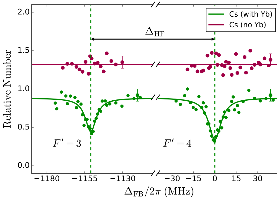
Figure 7.11: Observation of the photoassociation resonance for n' = -11 of ^{133}\text{Cs}^*^{174}\text{Yb} . Relative number of Cs atoms remaining after a 300 ms pulse of PA light versus detuning from the F' = 4 line ( \Delta_{\text{FB}} ). The green (red) trace shows the photoassociation spectra of Cs with (without) the presence of Yb in the dipole trap. The red (Cs only) trace has been offset for clarity. The statistical error in the atom number is shown by the error bars on the right hand side. The dashed green line shows the centres of the CsYb PA resonance for each hyperfine component.
