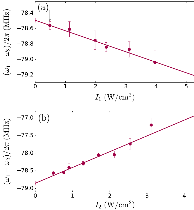
Figure 8.6: Light shift of the Cs 174 Yb n'' = -1 Raman line as a function of photoassociation laser intensity, using the n' = -13 intermediate state. (a) Measured line center frequency as a function of intensity I_1 of laser L_1 driving the free-bound transition. The intensity of laser L_2 for this data set was I_2 = 0.35 W/cm 2 . (b) Measured line center frequency as a function of intensity I_2 of laser L_2 driving the bound-bound transition. The intensity of laser L_1 for this data set was I_1 = 0.48 W/cm 2 and is highlighted in (a). The 1\sigma uncertainties in the intercepts are represented by the shaded regions at the origins.
