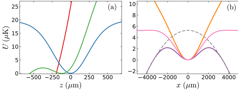
Figure 5.7: Effect of magnetic fields on the reservoir trap. Simulated optical potentials for the reservoir trap using Cs atoms in the |F = 3, m_F = +3\rangle state. For illustrative purposes the potential minimum has been set to zero for traps with a finite trap depth. (a) Trapping potential in the vertical direction for magnetic field gradients 0 G/cm (red), 24 G/cm (green) and 31 G/cm (blue). (b) Trapping potential in the axial direction for a levitating magnetic field gradient of 31 G/cm and magnetic bias fields 5 G (grey dashed), 70 G (purple), 100 G (pink) and 140 G (orange).
