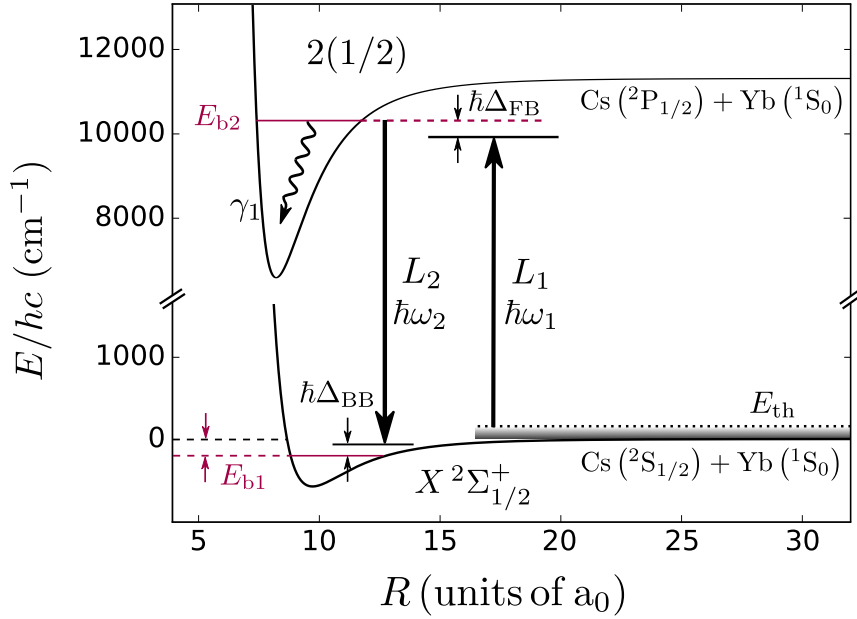
Figure 8.1: Two-photon photoassociation for the measurement of the binding energy, E_{b1} , of a vibrational level of CsYb in its electronic ground state. A pair of colliding Cs and Yb atoms with thermal energy E_{th} is associated to form a CsYb molecule in a rovibrational level of the electronically excited 2(1/2) state by light of frequency \omega_1 . This rovibrational level is coupled to a level in the electronic ground state, X^2\Sigma_{1/2}^+ , by light of frequency \omega_2 . The molecular curves plotted here are adapted from Ref. [300]. The internuclear distances where the transitions occur are not depicted to scale.
