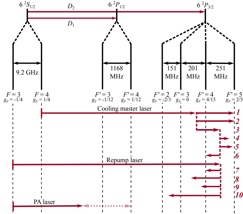
Figure 3.5: The upper section of the figure shows the energy levels of the D_1 and D_2 lines of Cs. The hyperfine states associated with each line are shown, with labels denoting the value of F and g_F factors [182]. The lower section of the figure shows schematically the approximate frequencies of the various Cs lasers and beams used in the experiment. The shorter arrows denote the frequency shifts given by AOMs and the red numbers label the AOM used to generate the required frequency: 1 is the imaging probe, 2 is the cooling spectroscopy. 3 is the BoosTA seed, 4 is the Zeeman slower cooling beam, 5 is the MOT cooling light, 6 is the DRSC lattice beams, 7 is the repump spectroscopy, 8 is the Zeeman slower repump light, 9 is the MOT repump light and 10 is the DRSC polariser light. The Cs photoassociation laser(s) (discussed in Chapters 7 and 8) are tunable to a broad range of frequencies red-detuned from the D_1 line.
