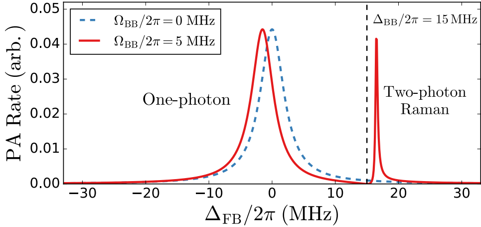
Figure 8.4: Photoassociation rate as a function of detuning from a one-photon photoassociation transition \Delta_{FB} for a bound-bound Rabi frequency \Omega_{BB}/2\pi = 0 MHz (blue dashed) and \Omega_{BB}/2\pi = 5 MHz (red solid). L_2 is detuned from the bound-bound transition by \Delta_{BB}/2\pi = 15 MHz, this detuning is shown by the dashed black line.
