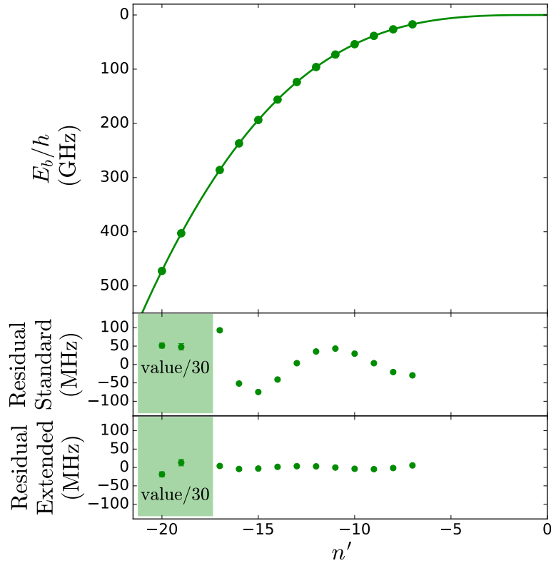
Figure 7.15: Binding energies of vibrational levels of ^{133}\text{Cs}^{174}\text{Yb} in the 2(1/2) excited state. Top: The binding energies as a function of the vibrational quantum number counted from dissociation, n' . The solid green line shows a fit to the data using the extended Le Roy-Bernstein equation. The lower two panels compare the residuals for the fits using the standard and extended Le Roy-Bernstein equations. The error bars are much smaller than the data points.
