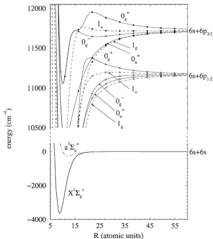
Figure 7.2: \text{Cs}_2 potentials near the ^2S+^2P_j asymptote. At long range the fine structure splitting is large compared to the Born-Oppenheimer interaction. Therefore, the multiple excited triplet molecular potentials are labelled using Hund's case (c). The ground state triplet ( a^3\Sigma_u^+ ) and singlet ( X^1\Sigma_g^+ ) potentials are labelled using Hund's case (a). From Ref. [303].
