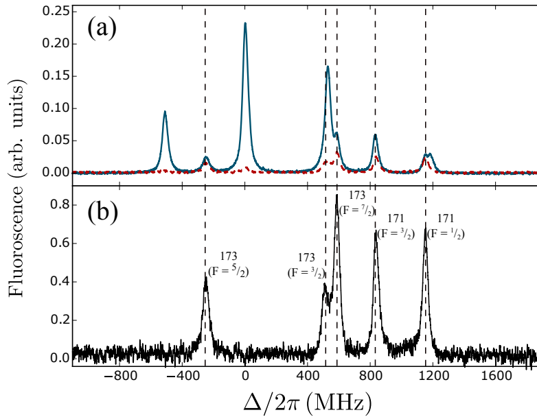
Figure 3.11: (a) The fluorescence spectrum of the ^1P_1 state for vertically (horizontally) polarised light is shown by the red (blue) line for a power P = 265 \mu\text{W} and temperature T = 470 \text{ }^\circ\text{C} . (b) Scaled difference of the two signals showing only the fermionic spectrum. The dashed vertical lines show the detunings measured by Das et al [200].
