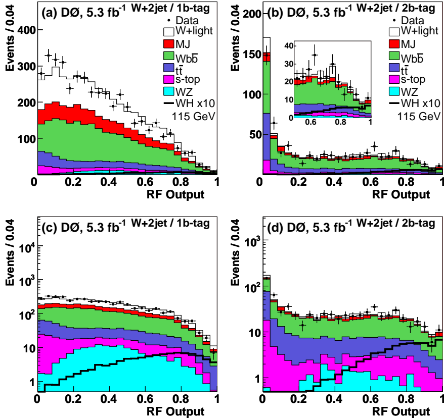
FIG. 10: [color online] Output RF distributions on linear and logarithmic scales for (a), (c) single (one- b -tag) and (b), (d) two- b -tagged W+2 jet events. The expectation for signal at M_H = 115 GeV (solid black line) is scaled by a factor of 10.
