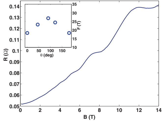
FIG. 8. (Color online) Typical oscillations in our lower carrier-concentration samples of n \sim 10^{17} \text{ cm}^{-3} . The inset is the typical 3D angular dependence of the oscillation frequency.
