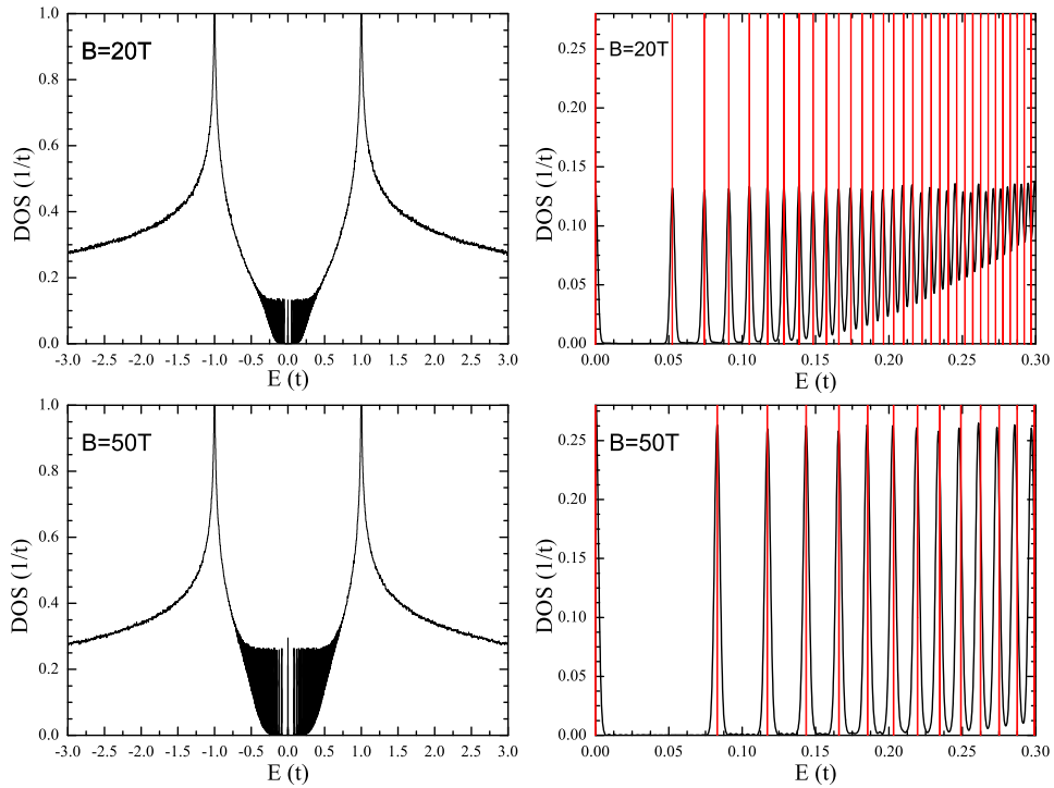
FIG. 2: Left: DOS of a monolayer of graphene in a magnetic field, for two different values of B . Right: zoom of the low energy region of the spectrum. The red vertical lines indicate the position of the LLs in the continuum Dirac cone approximation, Eq. (19). We have used a sample made of 4096 \times 4096 atoms.
