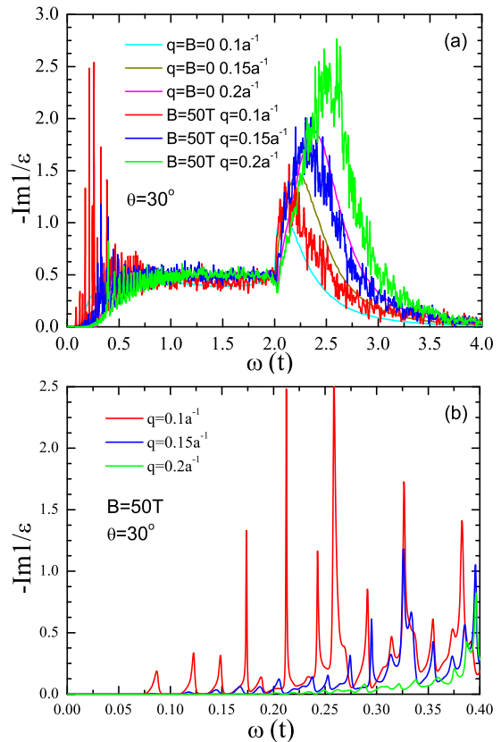
FIG. 5: (a) Loss function -\text{Im} 1/\epsilon(\mathbf{q},\omega) in the RPA, for different values of wave-vector. The results for graphene in a magnetic field of B = 50\text{T} are compared to the B = 0 case. (b) Zoom of the low energy part of the spectrum.
