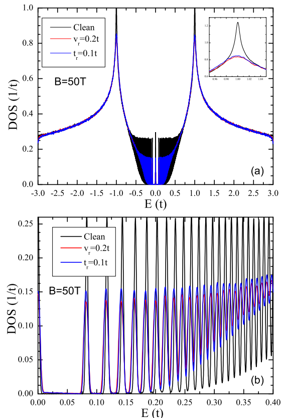
FIG. 7: (a) DOS of clean graphene (black lines) and of disordered graphene with a random on-site potential (red lines) and with a random renormalization of the hopping integrals (blue lines). The inset shows the smearing of the VHS peak due to disorder. (b) Zoom of the low energy part of the spectrum.
