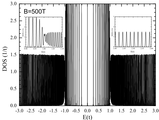
FIG. 3: DOS obtained from Eq. (4) at B = 500\text{T} . The insets show a zoom of the DOS around the VHS |\epsilon| \approx t and at |\epsilon| \approx 2.5t .
