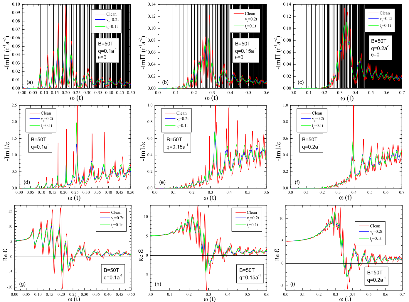
FIG. 8: (a)-(c) Non-interacting single-particle excitation spectrum of graphene in a magnetic field of B = 50\text{T} , as defined by -\text{Im}\Pi(\mathbf{q}, \omega) , for different kinds of disorder and for different values of the wave-vector q . The black vertical lines signal the energy of the electron-hole processes defined by Eq. (20). (d)-(f) Loss function -\text{Im}[1/\varepsilon(\mathbf{q}, \omega)] in the RPA. (g)-(i) Real part of the dielectric function \text{Re}\varepsilon(\mathbf{q}, \omega) in the RPA.
