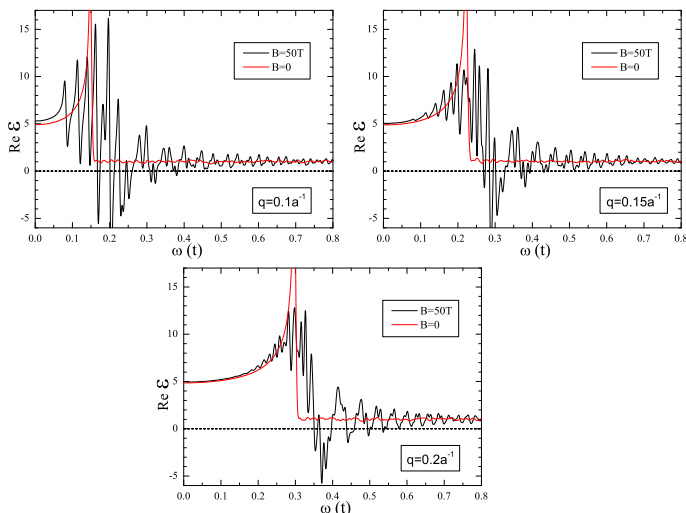
FIG. 6: \text{Re } \varepsilon(\mathbf{q}, \omega) for B = 0 (red lines) and B = 50\text{T} (black lines), for the values of the wave-vectors used in Fig. 5.
