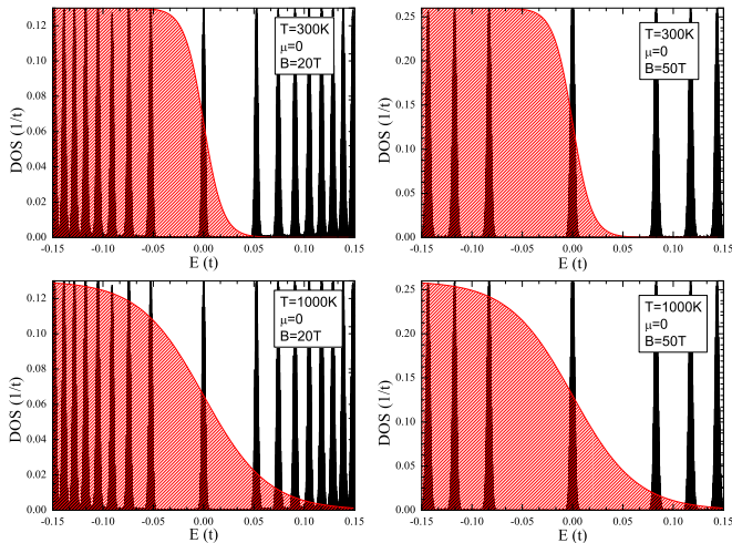
FIG. 9: DOS of clean graphene for different values of temperature T and magnetic field B . The shaded area is a sketch of the Fermi-Dirac distribution function for each case.
