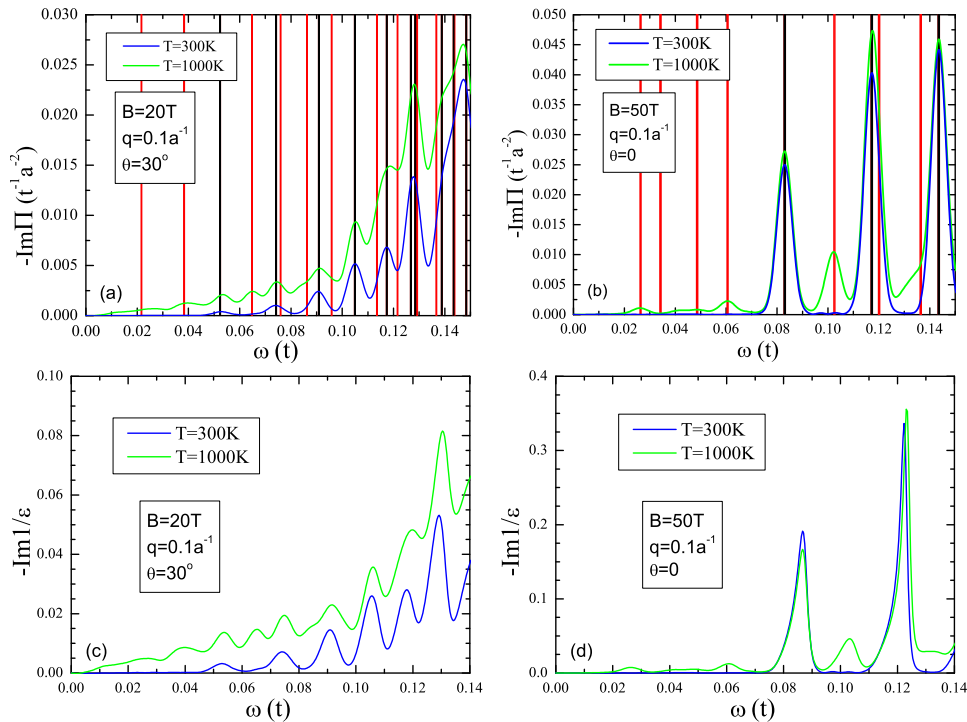
FIG. 10: (a)-(b) -\text{Im}\Pi(\mathbf{q}, \omega) for two different values of T and B . The black vertical lines denote the position of the inter-LL transitions given by Eq. (20) which are possible at T = 0 . The red vertical lines correspond to the energy of thermally activated inter-LL transitions. (c)-(d) Loss function -\text{Im}[1/\epsilon(\mathbf{q}, \omega)] for the same values of T and B .
