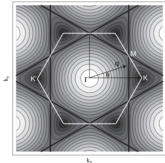
FIG. 1: Constant energy contours obtained from the band dispersion Eq. (13). The thick black lines correspond to dispersion at the VHS |\epsilon| = t . Notice that the CEC are centered around the Dirac points for |\epsilon| < t and around \Gamma for |\epsilon| > t . For illustrative reasons, the hexagonal BZ is shown in white. For undoped graphene, the valence and conduction bands touch each other at the vertices of the hexagon, the so called Dirac points (K and K'). The Van Hove singularity lies at the M point, and we have defined \theta as the angle between the wave-vector q and the k_x -axis.
