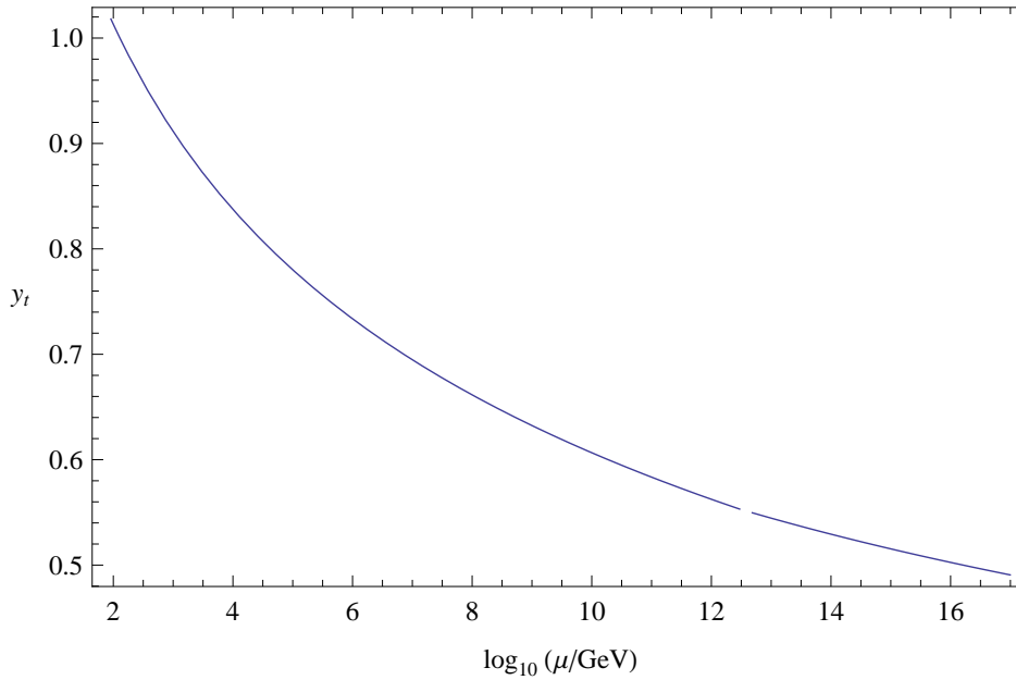
Figure 3: The running of the top-quark Yukawa coupling y_{\text{top}} for \Lambda_{GUT} = 9.92 \times 10^{16} GeV, \rho = 1.2 , and m_R = 3 \times 10^{12} GeV.
