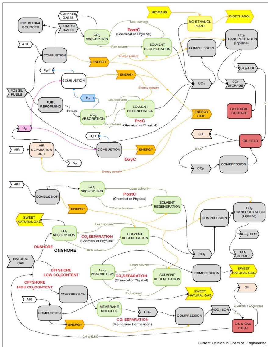
Fig. 8: Recent advancement of carbon dioxide capture routes [43]
