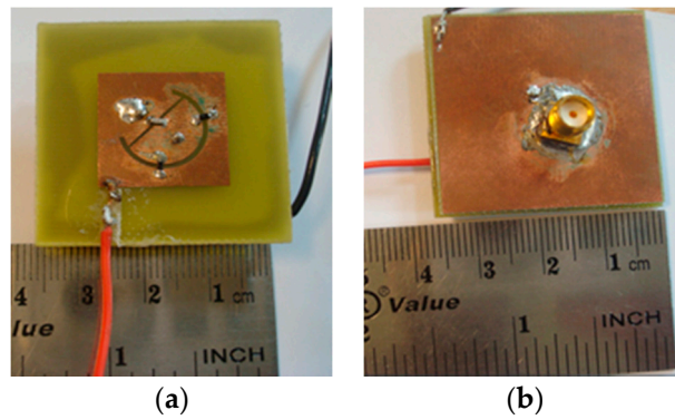
Figure 3. A photo of the fabricated antenna on a single FR-4 substrate. The red wire for (1 V) and black wire for (0 V) are used to control the diode states: (a) Top view; (b) Bottom view.
