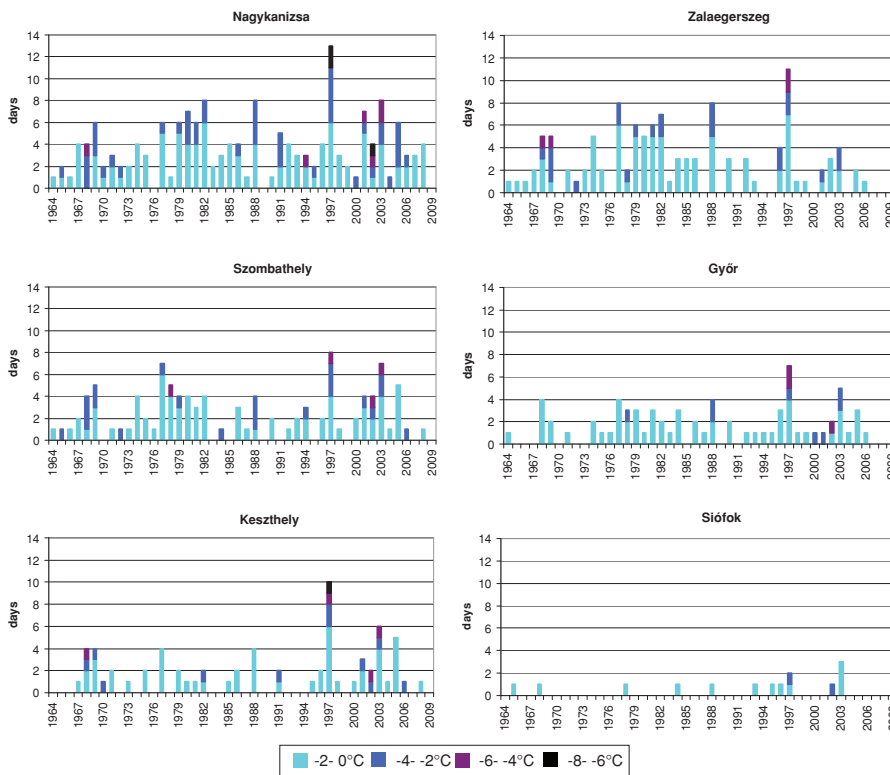
Figure 2. Number of frosty days in April
