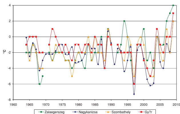
Figure 1. Absolute minimum temperatures in April
